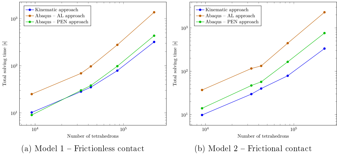
Figure 3.11 – Total solving time for each mesh size
