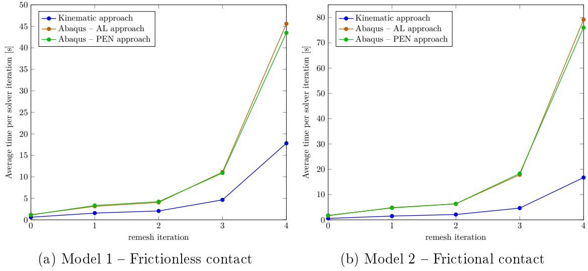
Figure 3.12 – Average solving time per internal algorithm iteration for each mesh iteration
