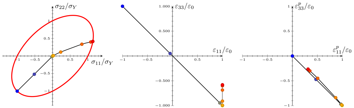
Figure 2.7 – Test 6 - Visualization of the different iterates
