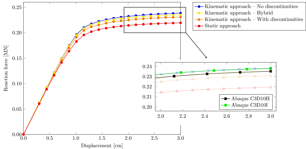
Figure 4.19 – Force-Displacement curves
