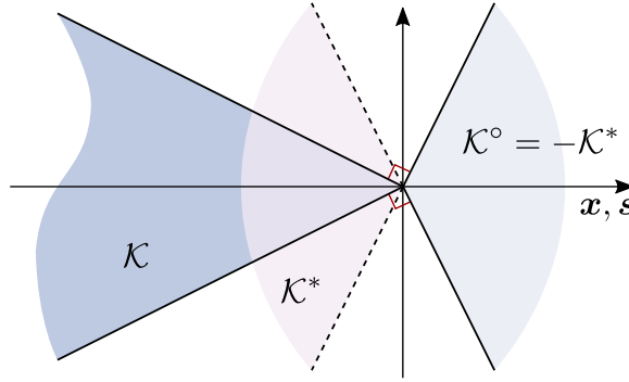
Figure A.1 – Primal, polar and dual cones
