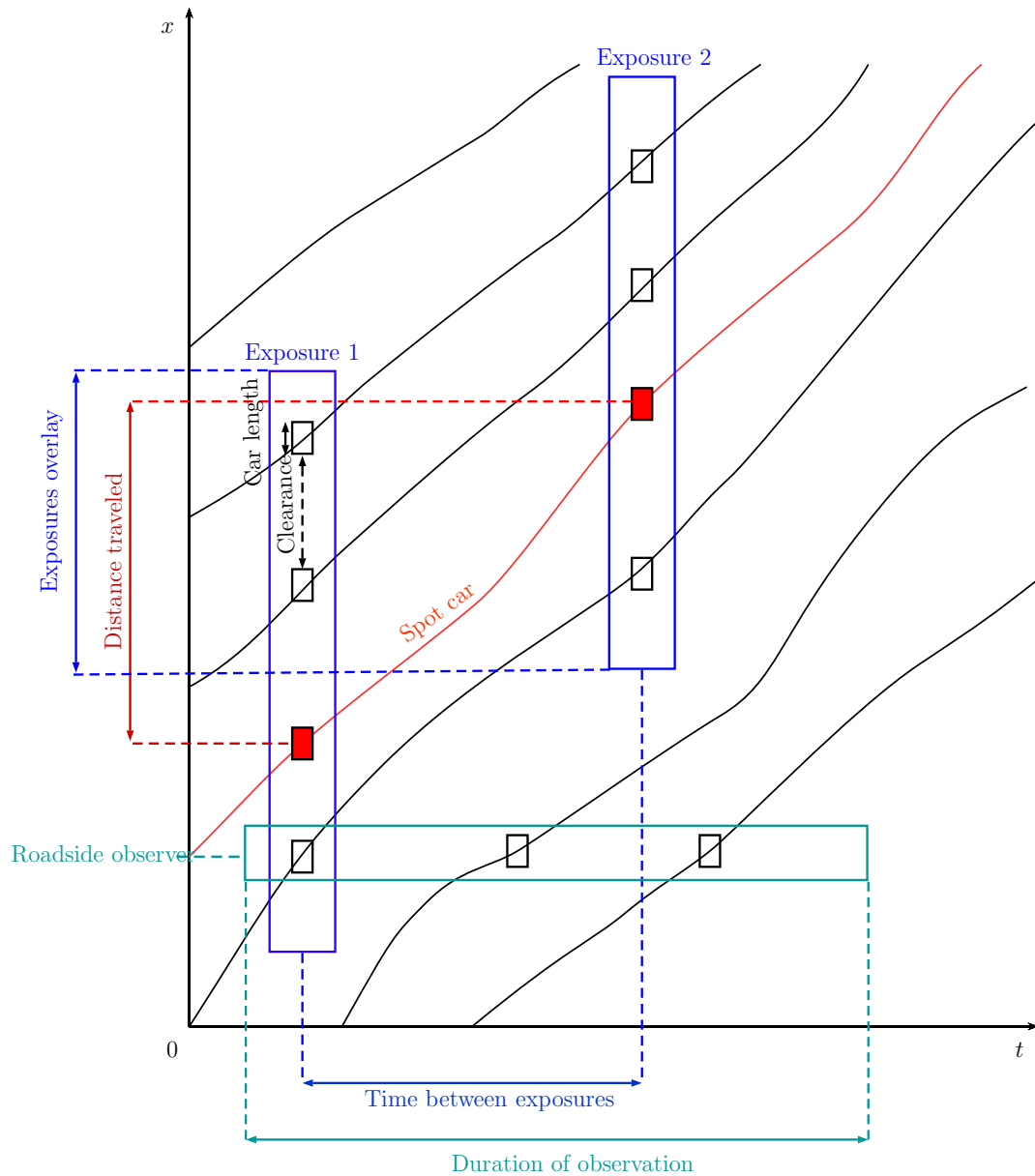
Figure 2.1 – Traffic variables at stake in Dean A.N. JOHNSON’s traffic study [17], drawn upon an x - t diagram.
