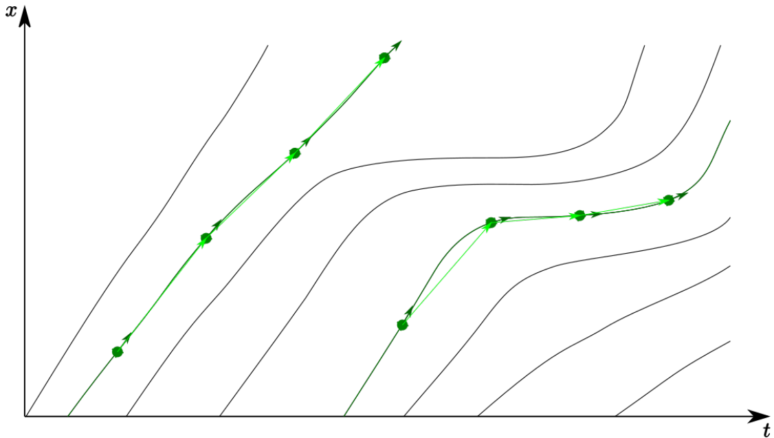
Figure 19 – Time-space t - x diagram showing traffic viewed by GPS-equipped vehicles, the dots representing the sampling of the equipped vehicles’ trajectories at regular \delta t -long intervals. For each trajectory and position, the dark green arrow represents the instantaneous speed, whereas the light green arrow represents the positional speed, i.e. the average speed between two successive GPS positions.
