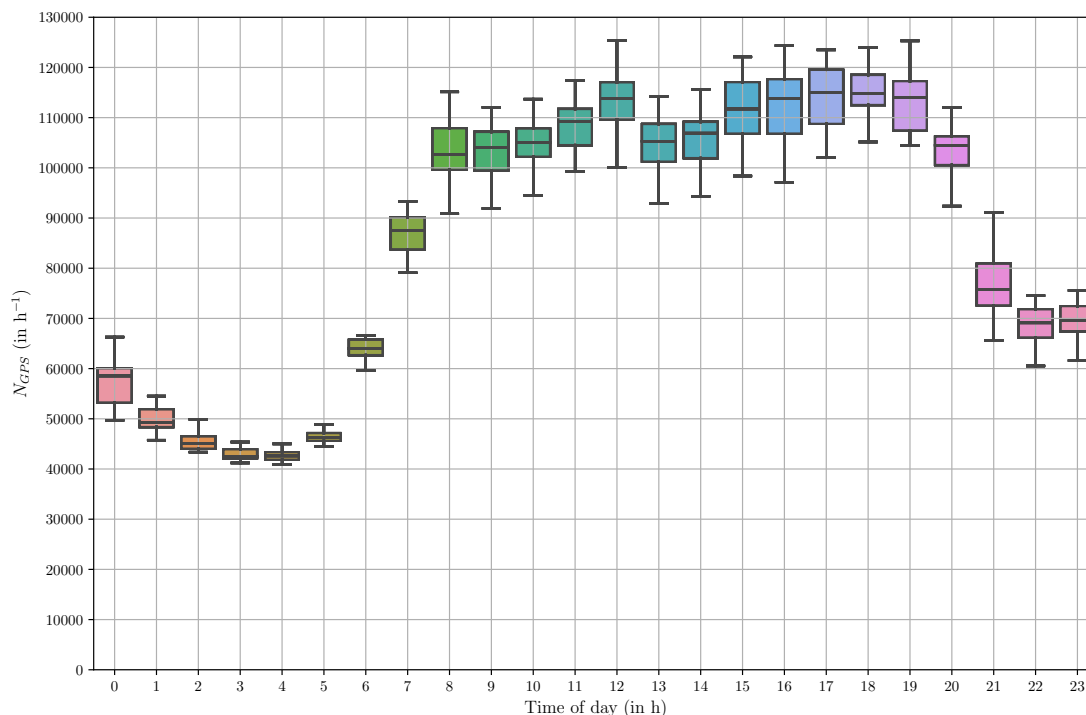
Figure 6.7 – Provider 1. First delivery. Distribution of Number of Positions N_{GPS} computed per hour and per day, over TPIM. Business days of October 2014.
