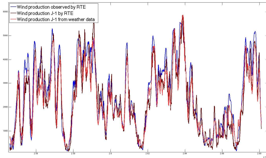
Figure 2.3.7: All curves are hourly production data. The origin of the hours is the first of January 2011, and the production is in MWh. In blue: the observed wind production. In dark red: the day-ahead predictions from the grid operator. In light red: the day-ahead predictions from weather data.
