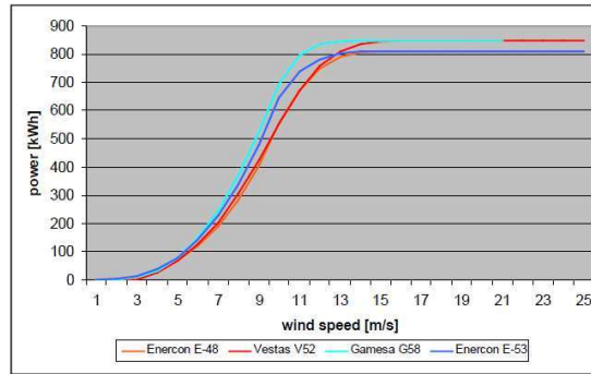
Figure 2.3.6: Typical response curves of different wind turbines
