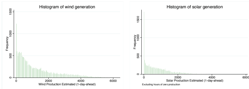
Figure 3.B.5: Histogram of predicted wind (left) and predicted solar (right) generation
