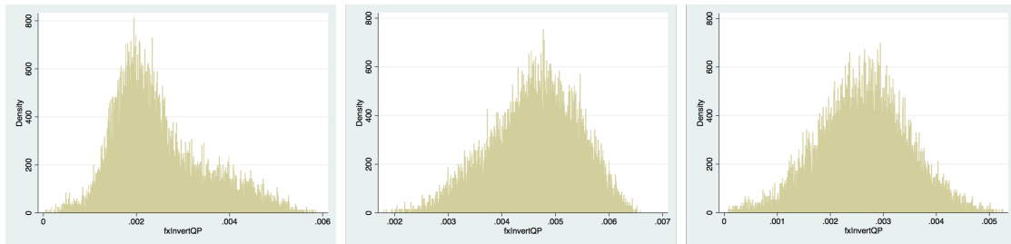
Figure 2.2.6: Histogram of slopes per point type
