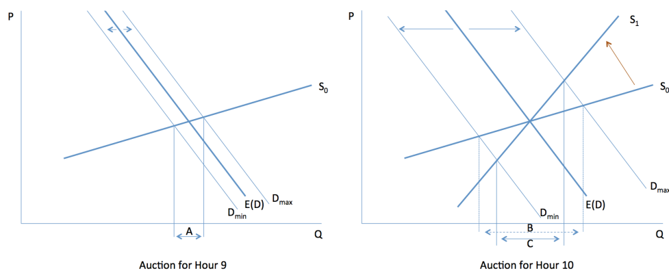
Figure 3.1.1: Illustrating the effect of increased uncertainty.
