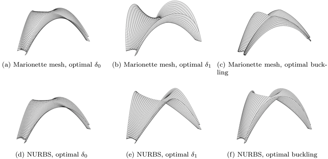
Figure 6.28 – Geometry of the best optima for each objective ( \frac{t}{L} = \frac{1}{250} )
