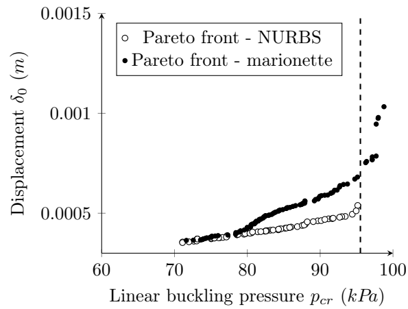
Figure 6.18 – Comparison of the Pareto fronts (p_{cr}, \delta_0) of the two design spaces.
