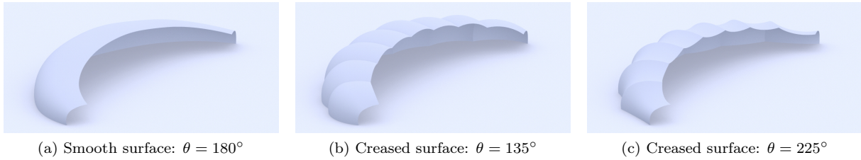
Figure 4.44 – Three different generalised cyclidic nets supported on the same circular mesh.
