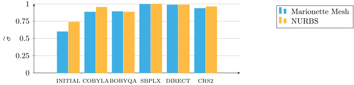
Figure 6.11 – Optimal values found for the minimisation of the maximal tensile stress under self-weight.
