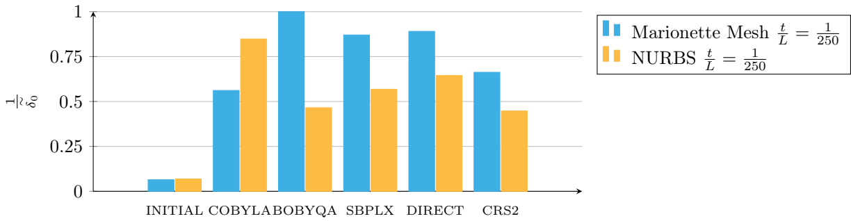
Figure 6.25 – Optimal values found for the minimisation of displacement under self-weight ( t/L = 1/250 ).
