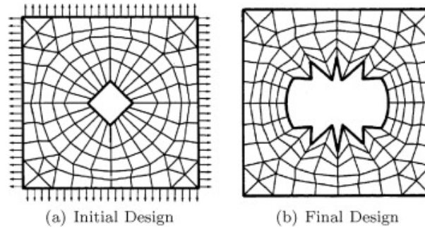
Figure 6.1 – Result of optimisation of a plate with a hole with a node-based parametrisation [46]
