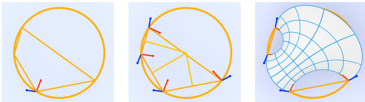
Figure 4.3 – Cyclidic patch: the four corners are on the same circle, the surface is naturally parameterised by its lines of curvature. The frames define tangent vectors for the edges of the patch.
