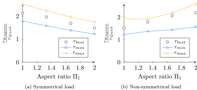
Figure 7.19 – Comparison of the structural performance of domes.
