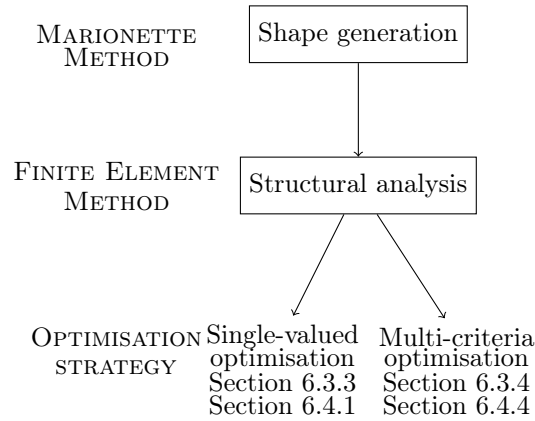
Figure 6.2 – Framework for the shape optimisation of shells
