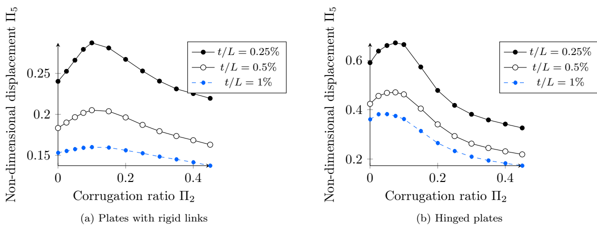
Figure 7.44 – Non-dimensional displacements vs. corrugation ratio ( h/L = 0.15 ), RT strategy
