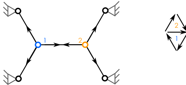
Figure 2.20 – A network at equilibrium (form-diagram) and the corresponding force-diagram (right).
