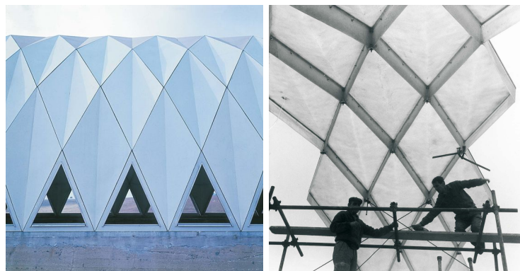
Figure 7.24 – An example of folded plate structures: Sulfur Extraction Facility (arch.: Renzo Piano, retrieved from compositesandarchitecture.com )
