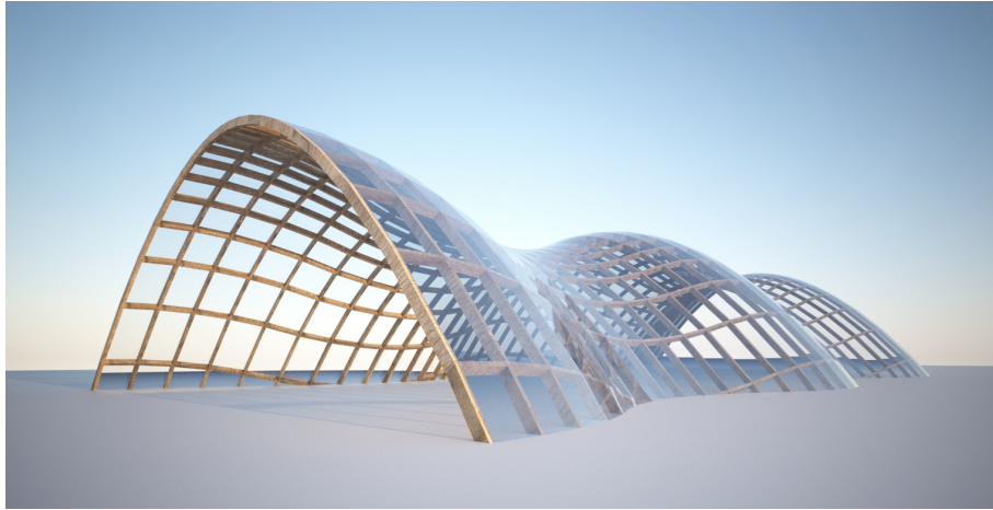
Figure 3.5 – Free-form generated as an isogonal moulding surface.
