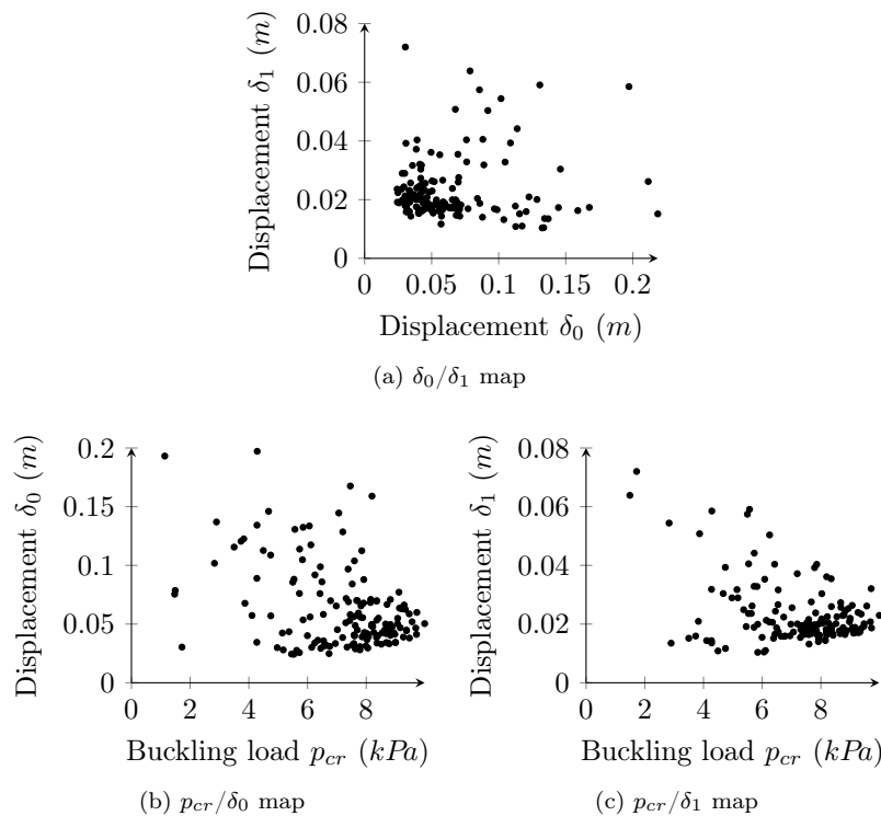
Figure 6.30 – Pareto front for three objectives for the NURBS design space for the shell with t/L = 1/1000 .
