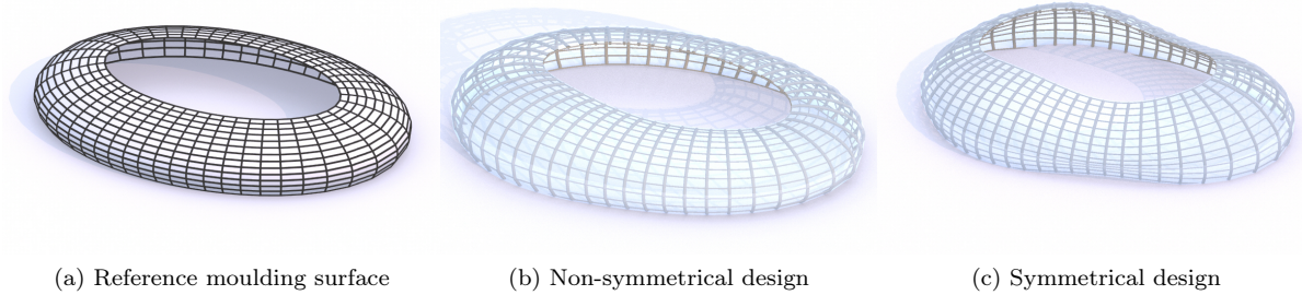
Figure 5.18 – Design of stadia obtained from a projection on a moulding surface: the prescribed curves are the inner ring and a section curve.
