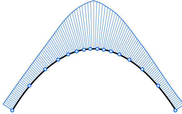
Figure 3.22 – Curvature graph of the rail curve in Figure 3.21, the dots represent the tangency points found with the algorithm presented in this paper.
