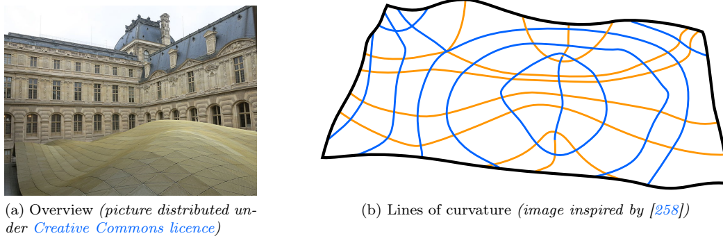
Figure 1.6 – Roof spanning over the Visconti court in Le Louvre museum (architect: Rudy RICIOTTI and Mario BELLINI).
