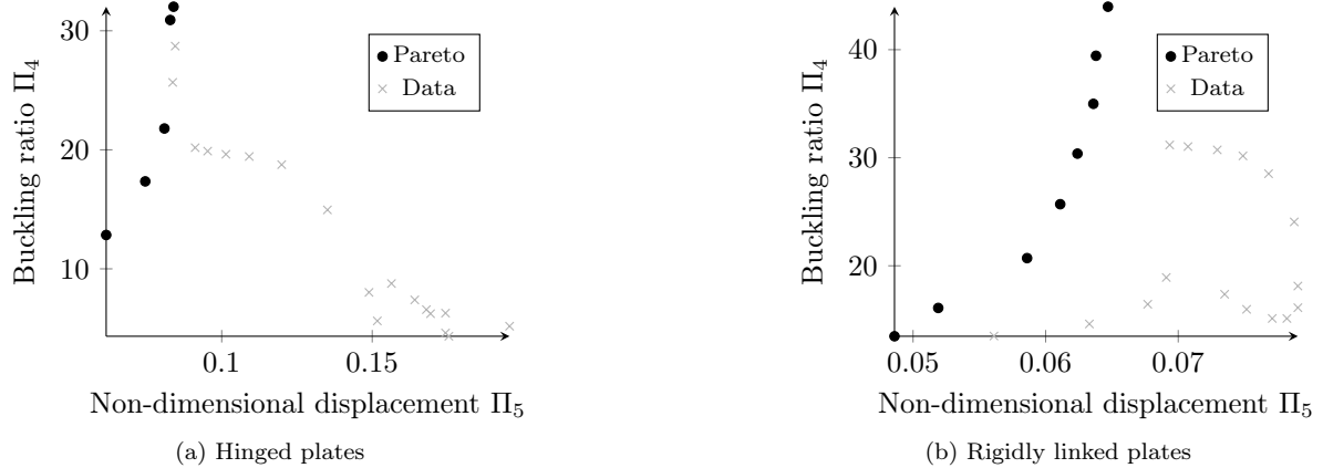
Figure 7.45 – Pareto frontier for the open dome, t/L = 1\% , AT strategy
