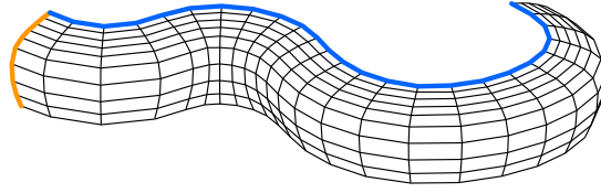
Figure 3.7 – A vertical doubly-curved facade as an isogonal moulding surface, all the generatrices are equal.
