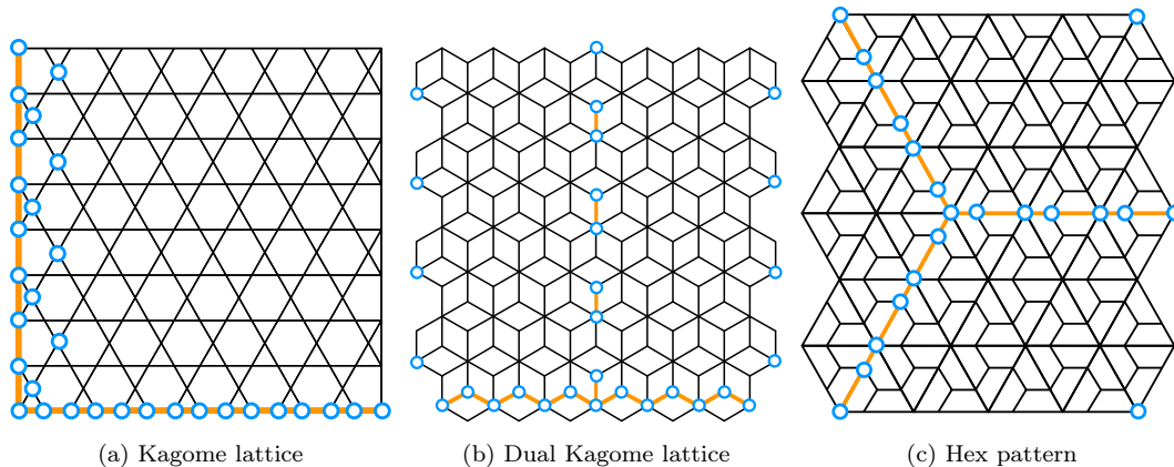
Figure 5.19 – Marionette method applied to several patterns, white dots correspond to prescribed altitudes.
