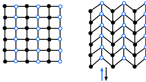
Figure 7.26 – RT strategy for the generation of 'Miura Ori' (herringbone) pattern.
