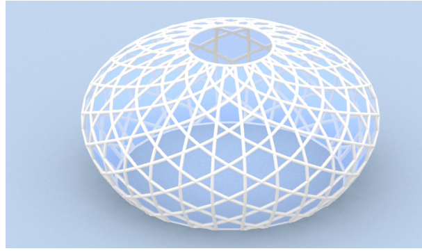
Figure 5.21 – A Kagome grid pattern covered with planar facets generated with the method described in this section.
