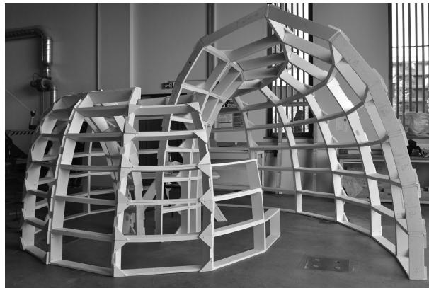
Figure 4.42 – A pavilion built with torsion free-nodes on a super-canal surface.
