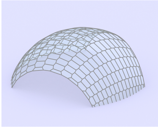
Figure 4.1 – A surface covered with planar hexagons, the panels layout follows lines of curvature.
