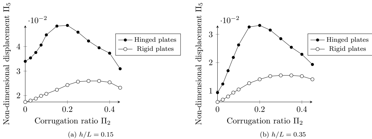
Figure 7.34 – Non-dimensional displacement vs. corrugation factor ( t/L = 1\% , AT strategy)
