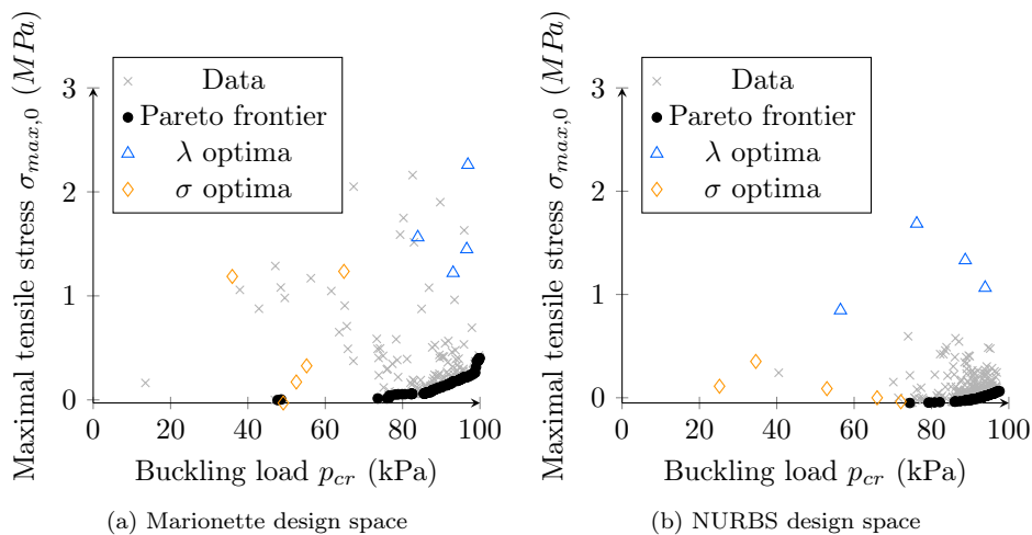
Figure 6.14 – Multi-criteria optimisation
