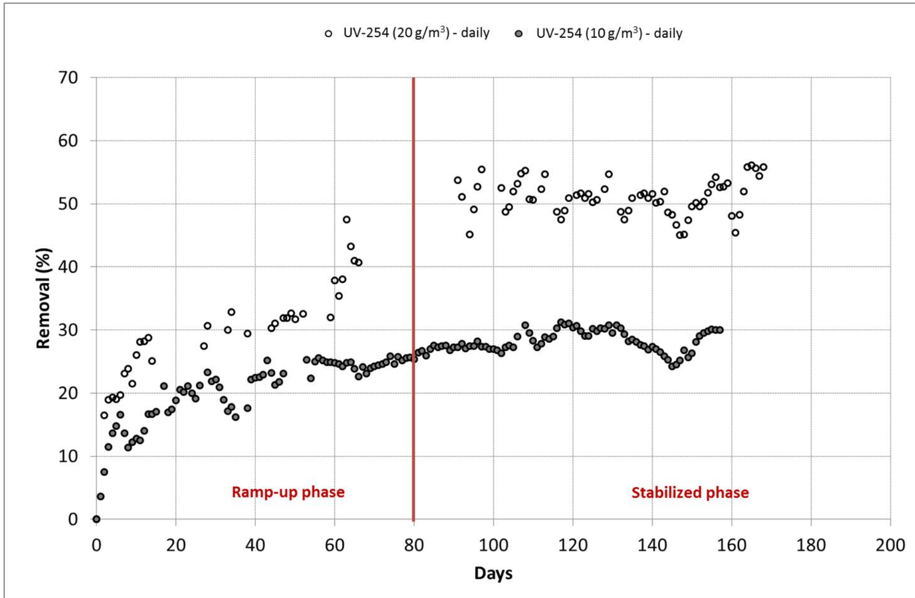
Figure III-15 : Ramp-up phase of the \mu\text{GAC} fluidized bed pilot for both assessed doses (10 and 20 \text{g}_{\mu\text{GAC}}/\text{m}^3 )
