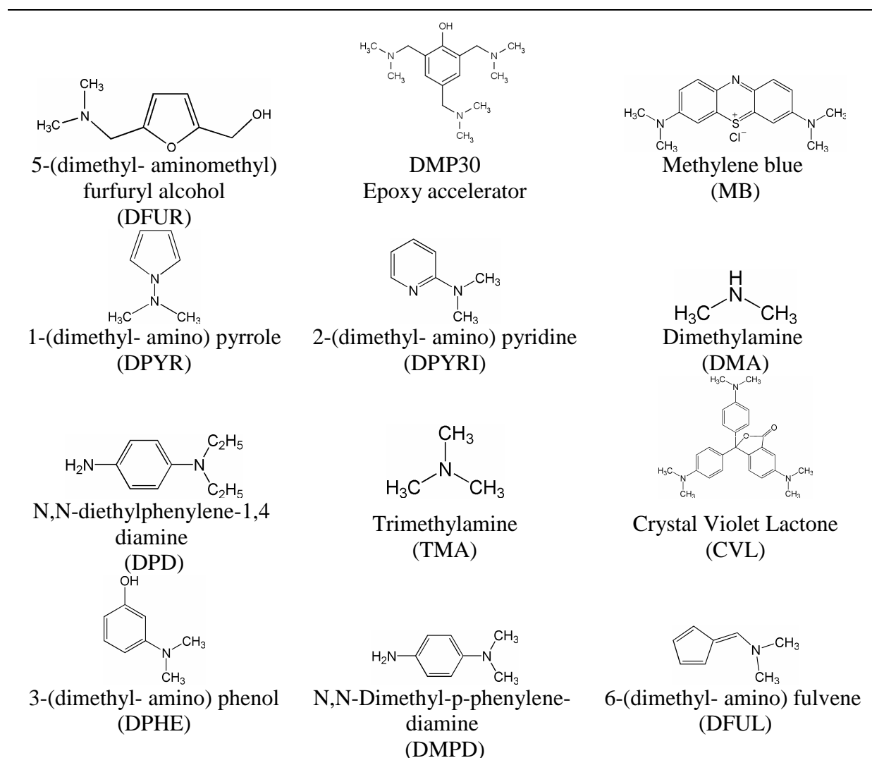
Figure III.C.1. Molecular structures of investigated compounds
