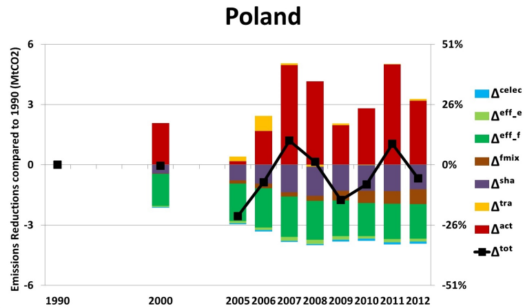
Figure 4.15: LMDI decomposition analysis of cement emissions compared to 1990. Poland
