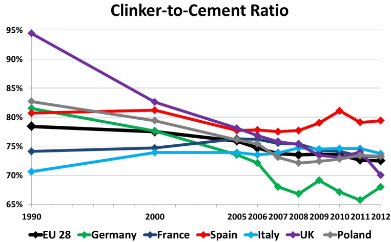
Figure 4.1: Clinker-to-cement ratio for the EU 28 and main European countries. Source: WBCSD GNR Database, variable 3213
