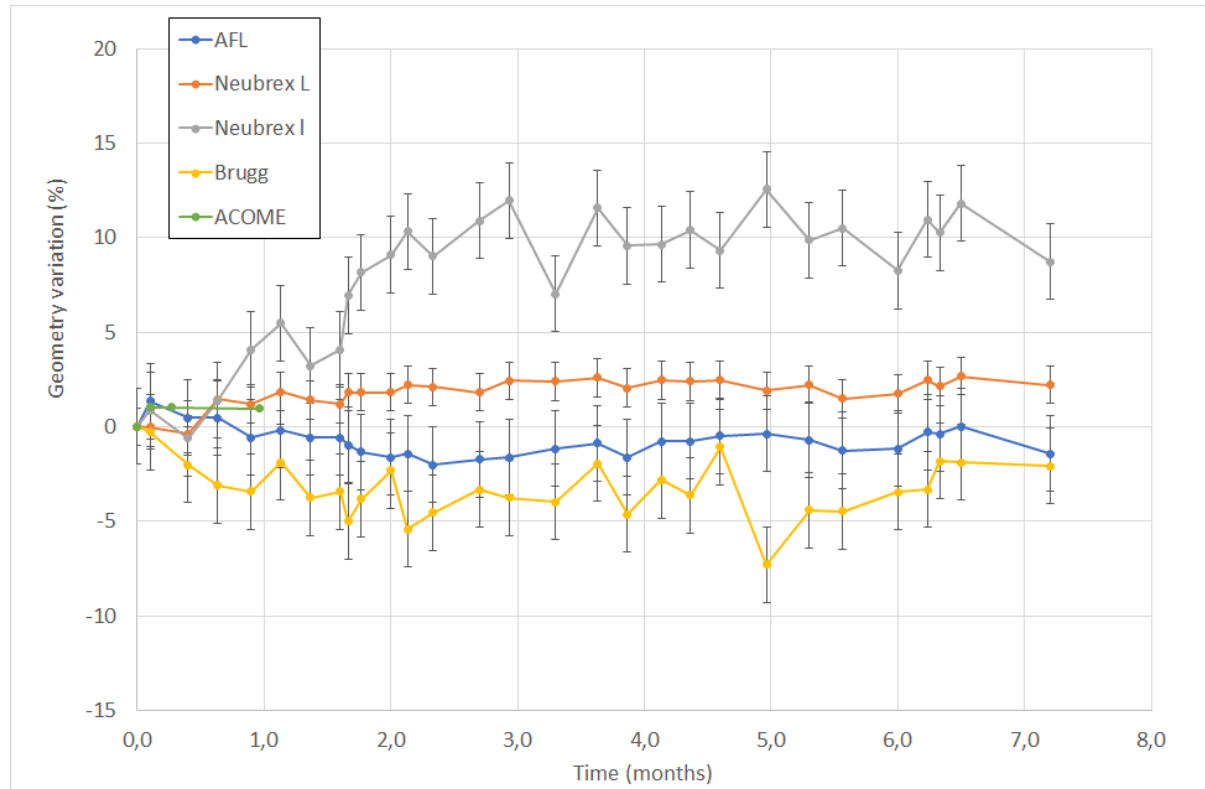
Figure 14. Dimensional changes of cables used for instrumentation in VeRCoRs mockup during exposure to alkaline solution at 60°C. 'L' and 'I' denote the larger and smaller lengths, respectively, of the rectangular section of the Neubrex cable.
