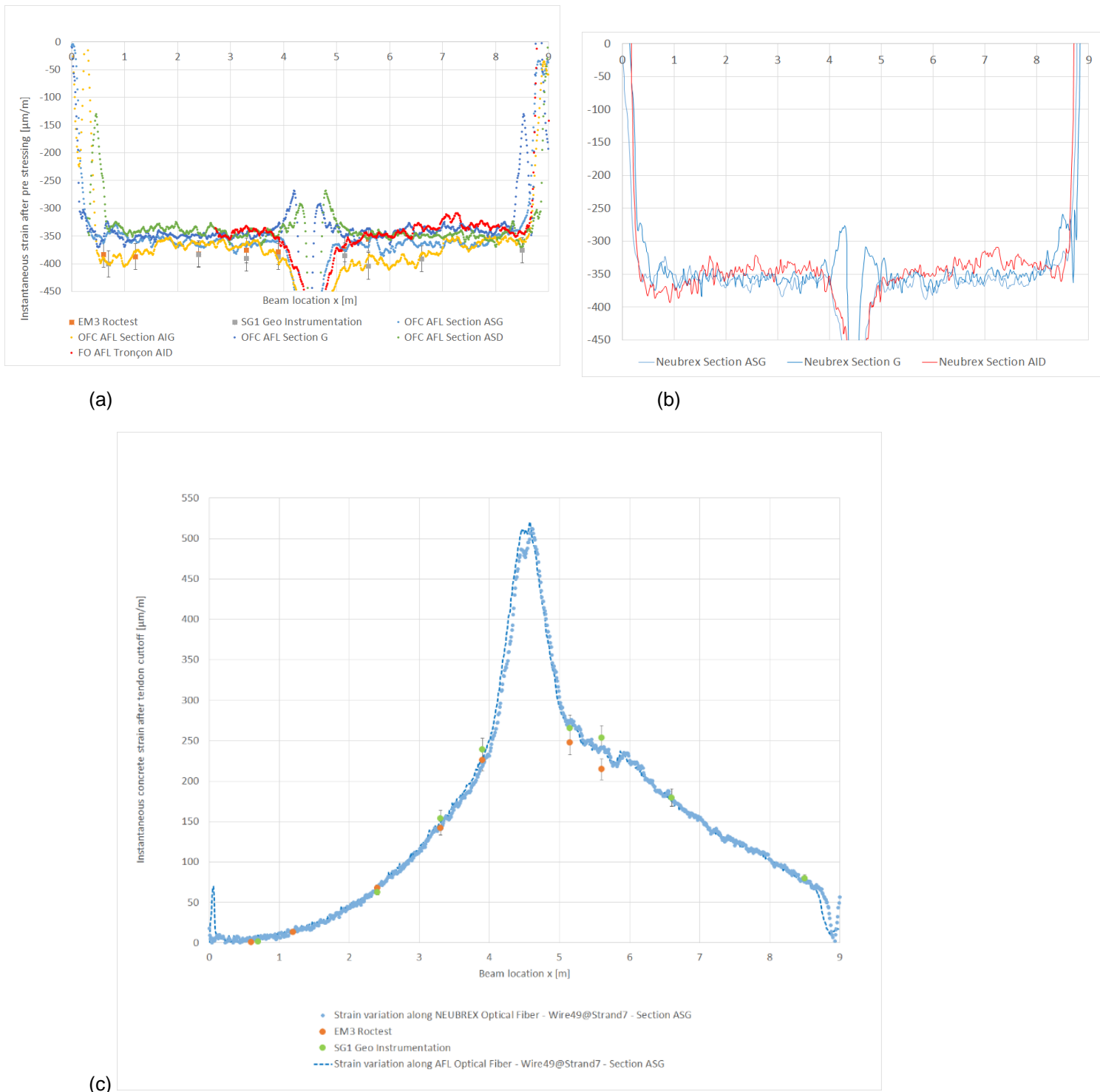
Figure 18: Instantaneous concrete strain profile along the beam length measured after tendon tensing with AFL (a) Neubrex (b) cables, and after tendon cutting with both OFC (c).
