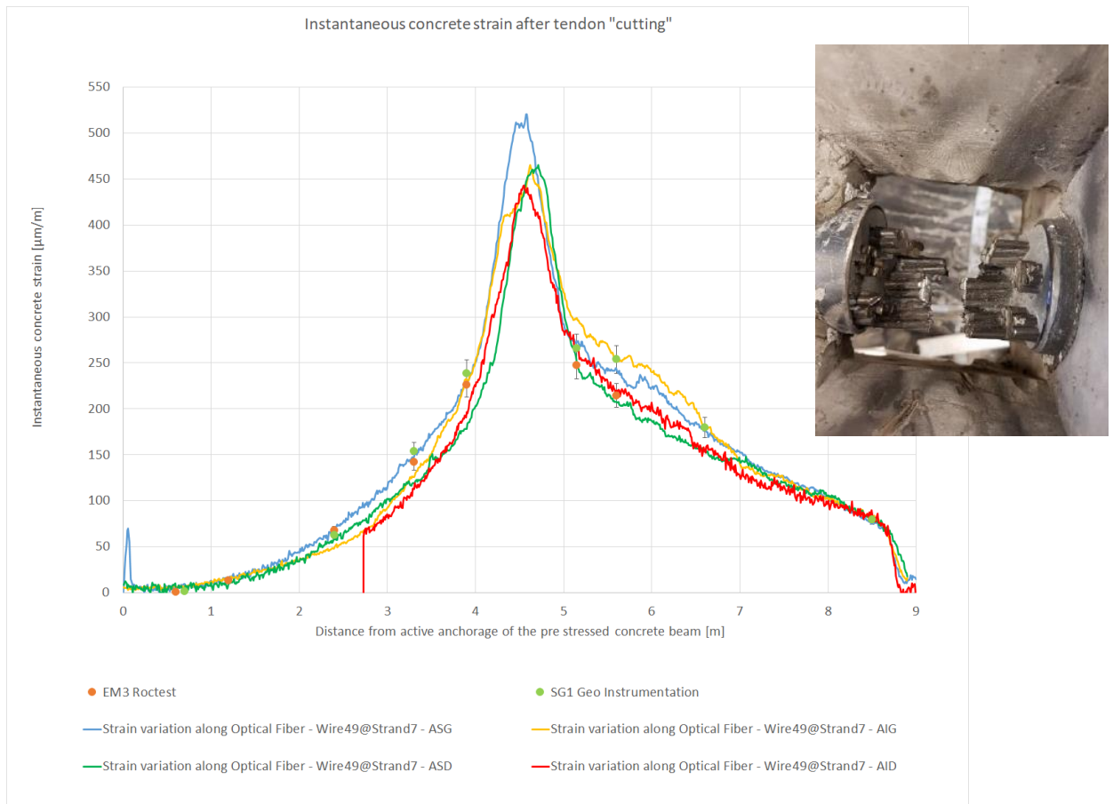
Figure 16: Concrete strain profile along the beam length after tendon cutting – comparison of OFC and VWSG measurements. The enclosed image shows the aspect of the cut tendon.
