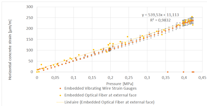
Figure 6. Concrete strain measured with VWSG and Embedded Optical Fiber [µm/m] versus pressure [MPa], at the mid height of the containment during SIT N°6
