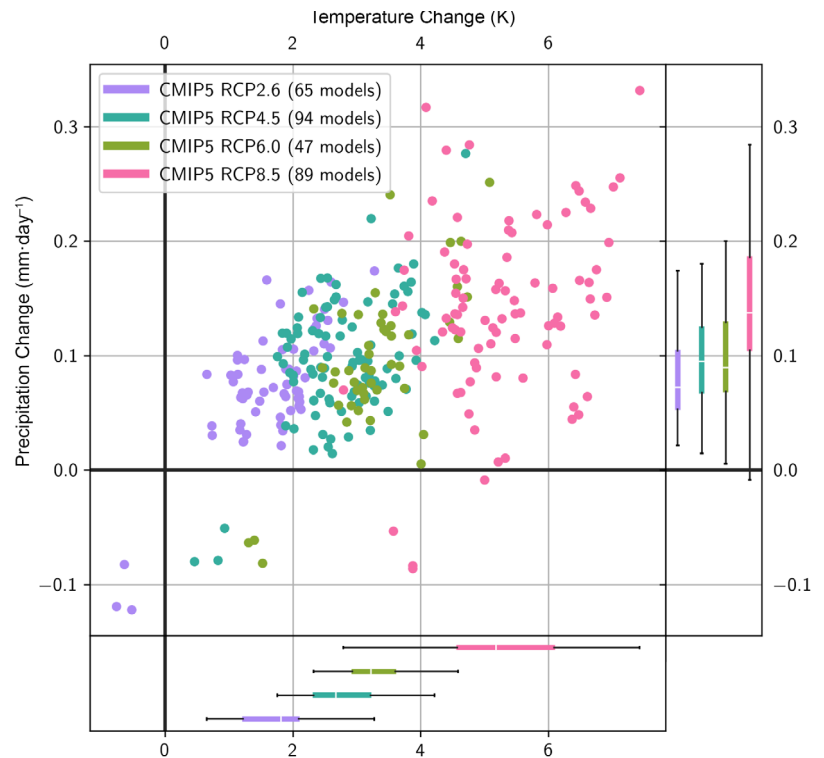
(a) CMIP5
