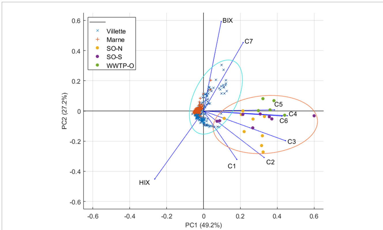
FIGURE 6 PCA of PARAFAC components, HIX and BIX, with dataset of La Vilette basin (blue, n = 183 ), Marne (orange, n = 207 ), SO-N (yellow, n = 9 ), SO-S (purple, n = 8 ), and WWTP-O (green, n = 5 ). Blue ellipse groups watercourses samples (La Vilette basin and the river Marne) and orange ellipse the SO and WWTP-O.
