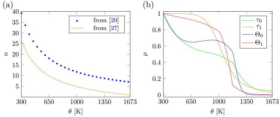
Figure 2: (a) Power law exponent n from [29] and [27] plotted as a function of \theta . The orange solid curve is used in this work. (b) Multiplication factor \mu(\theta) for the Voce parameters plotted as a function of \theta using the data obtained from [34].
