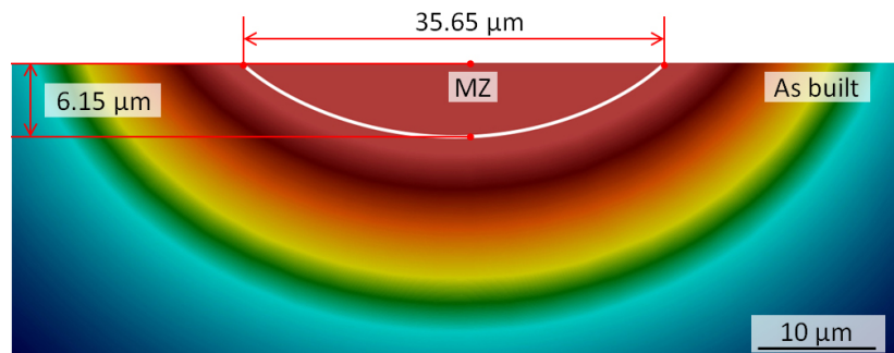
Figure S3: Cross-sectional view of the temperature field depicting the simulated melt pool.
