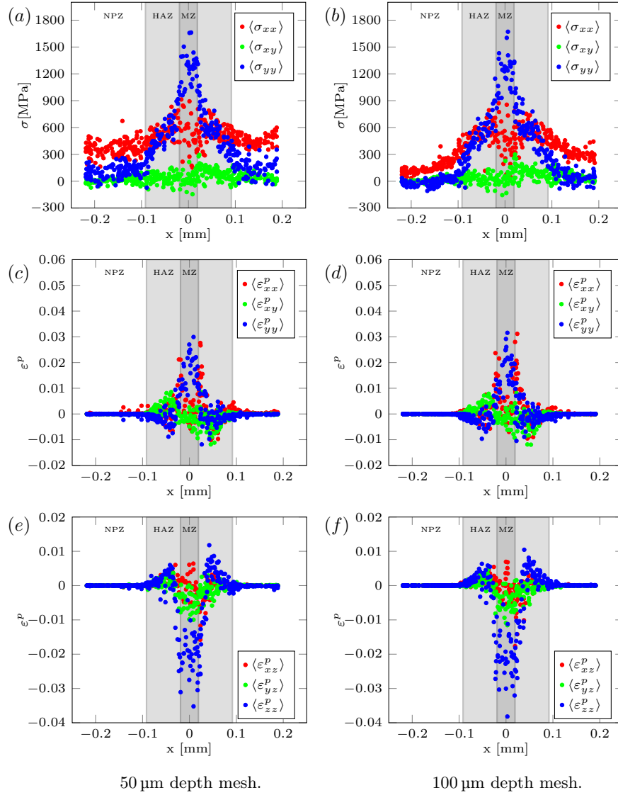
Figure S5: Residual stress and plastic strain components averaged on the top surface over each grain plotted as a function of the distance along x from the center of the laser scan path for the 50 \mu\text{m} and 100 \mu\text{m} depth microstructures. The residual state MZ, HAZ and NPZ are demarcated using grey shaded or unshaded regions.
