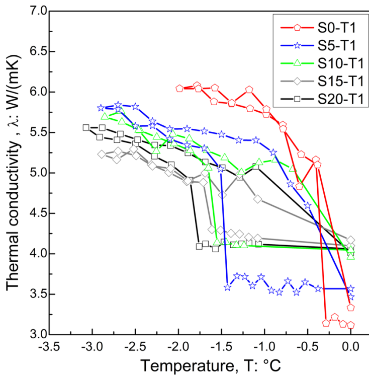
274 275 Fig. 6. Thermal conductivity versus temperature for all freezing-thawing experiments.
