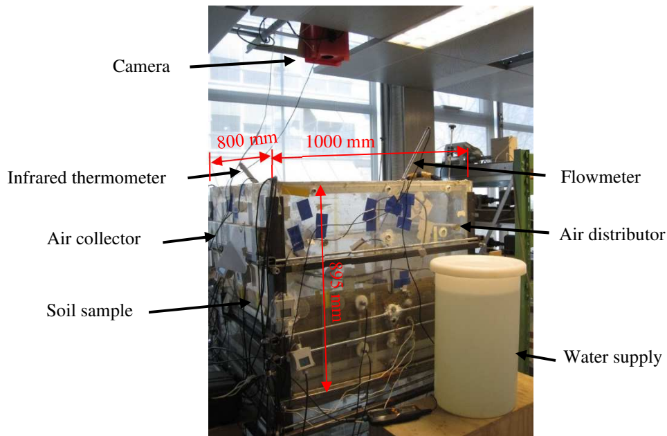
Figure 1. Environmental chamber used for evaporation experiment (modified from Song et al. 2013)
