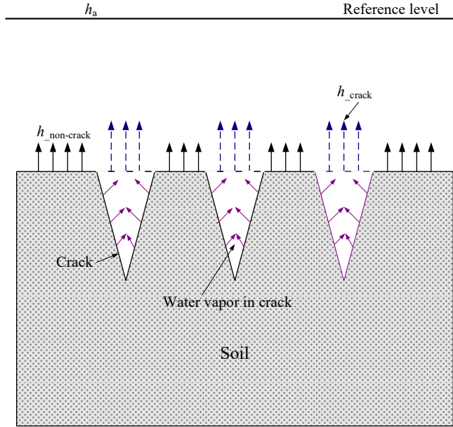
Figure 9. Sketch of water evaporation from cracked clay (modified from Song et al. 2020)
