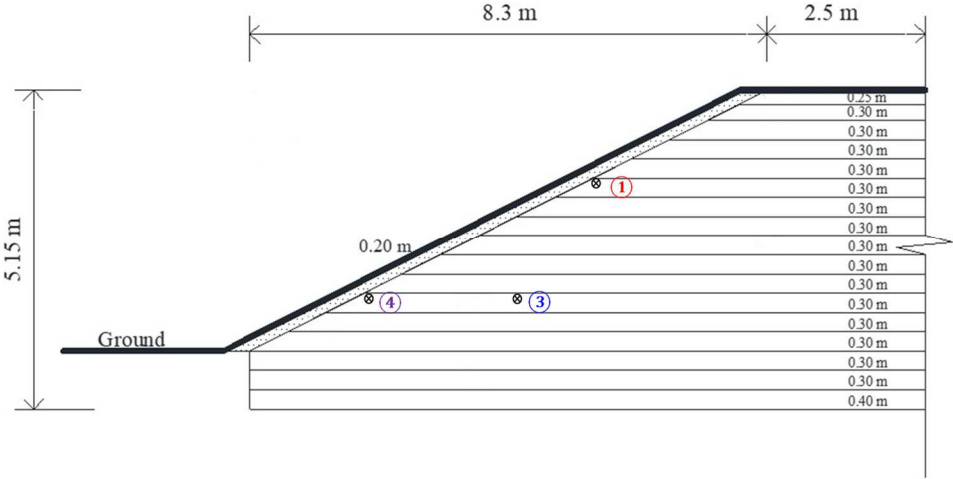
Figure 14. Points considered in the numerical analysis (modified from An et al. 2017b)
