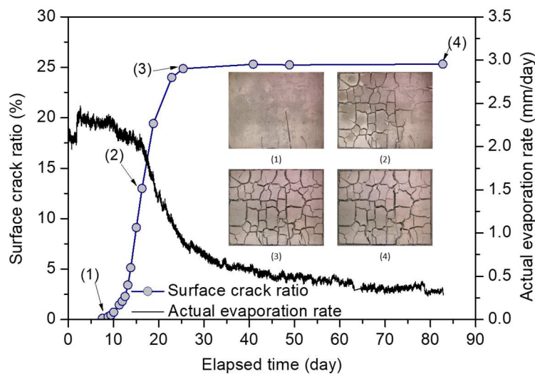
Figure 8. Evolutions of actual evaporation rate and surface crack ratio (data from Song et al. 2016)
