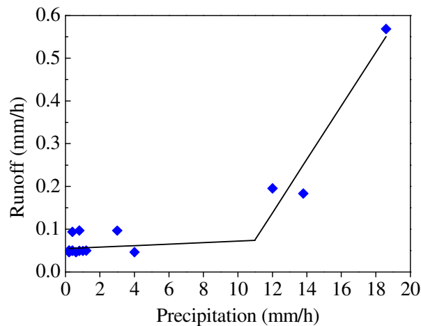
Figure 13. Runoff measured on the side slope versus precipitation (data from An et al. 2017a)
