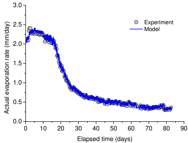
Figure 10. Comparison between the measured and predicted actual evaporation rates
