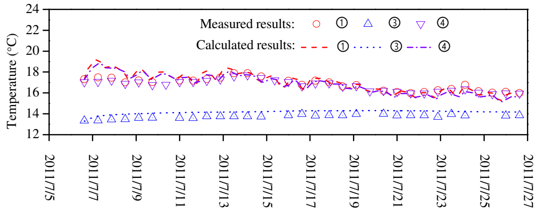
Figure 15. Comparison of temperature changes between calculation and measurement (data from An et al. 2017b)
