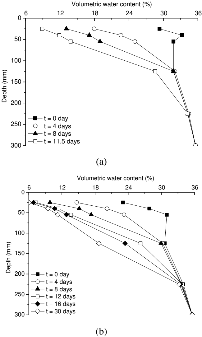
Figure 3. Volumetric water content profiles. (a) test 1 and (b) test 2 (data from Song et al. 2014)
