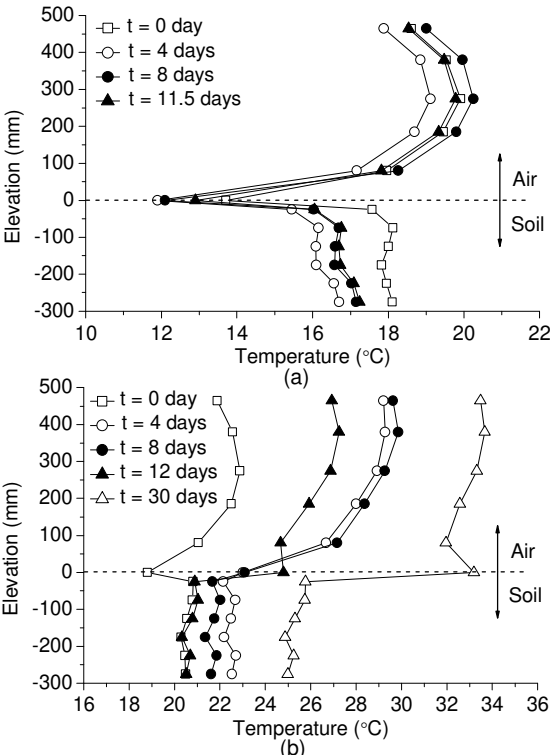
Figure 2. Temperature profiles in air and soil. (a) test 1 and (b) test 2 (data from Song et al. 2014)
