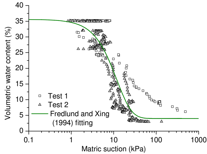
Figure 5. Water retention curve determined using data of volumetric water content and suction from tests 1 and 2 (data from Song et al. 2014)
