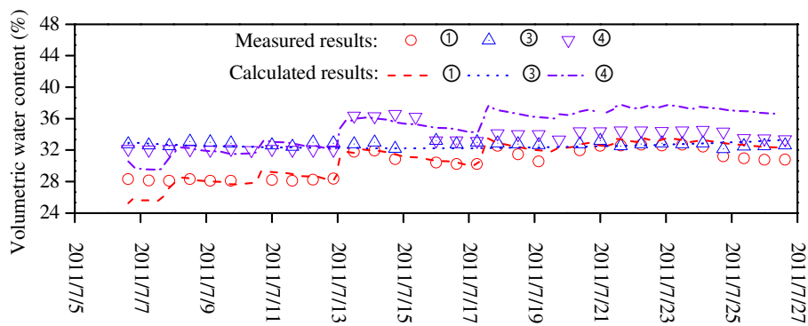
Figure 16. Comparison of changes in volumetric water content between calculation and measurement (data from An et al. 2017b)
