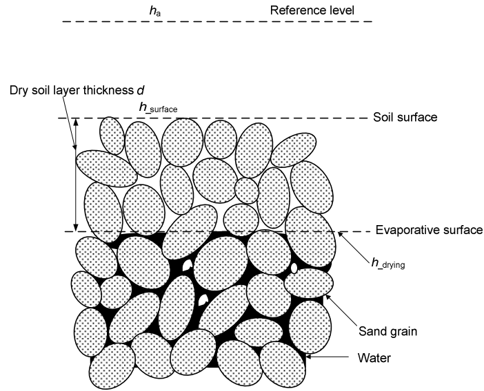
Figure 7. Evaporation with a dry layer (modified from Song et al. 2018)
