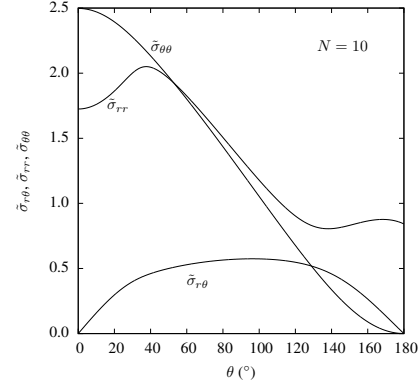
FIGURE 6.9: Functions \tilde{\sigma}_{r\theta} , \tilde{\sigma}_{rr} , \tilde{\sigma}_{\theta\theta} as functions of \theta for N = 10 .
