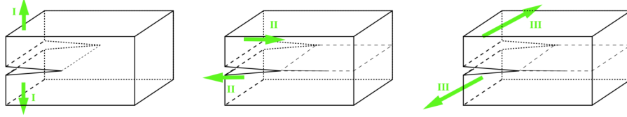
FIGURE 5.3: Three fracture modes: mode I for tensile crack, mode II for plane-shear, mode III for antiplane shear
