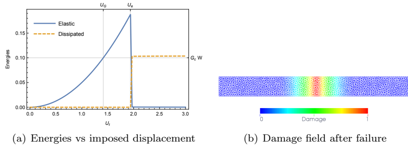
FIGURE 12.4: Numerical simulation of the traction test using the AT1 model ( E_0 = 1.0 , G_c = 1.0 , \ell = 0.1 ) for a bar of length L = 1.0 and width W = 0.1 . The vertical gridlines denote the analytically calculated elastic limit t = U_e = L\sqrt{3G_c/8E_0\ell} = \sigma_c L/E_0 and critical Griffith loading t = U_G = \sqrt{2G_c L/E_0} ; the horizontal gridline is the dissipated energy for a transverse crack according to the Griffith model.
