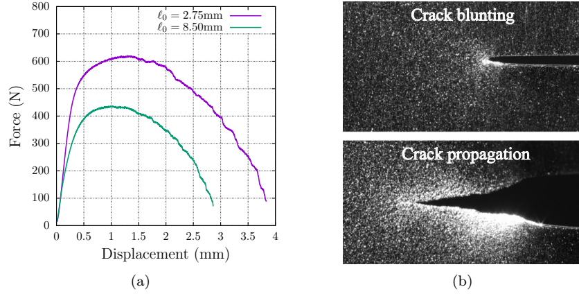
FIGURE 4.14: (a) Force-displacement curves for different initial crack lengths \ell_0 , for a thickness h = 0.1 mm (b) Crack evolution: blunting then propagation
