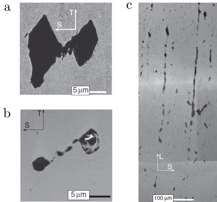
FIGURE 9.8: Three main modes of coalescence. (a) Coalescence by internal necking (also know as coalescence in layers) [Benzerga et al., 1999]. (b) Coalescence in shear [Benzerga, 2000]. (c) Necklace coalescence (also known as coalescence in columns) [Benzerga, 2000]. In the three cases considered, the loading is vertical.
