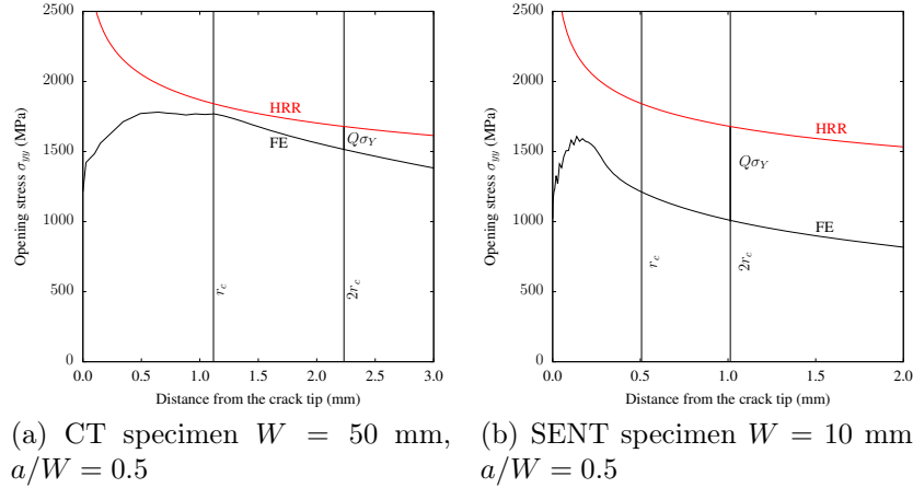
FIGURE 6.14: Evaluation of the Q -factor for (a) a CT specimen and (b) a SENT specimen. J = 294 \text{ kJ/m}^2 .
