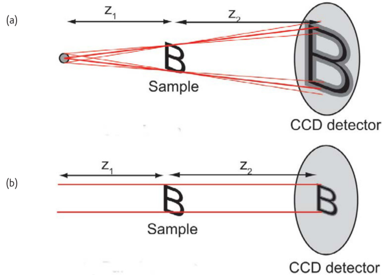
FIGURE 8.19: Schematics illustrating (a) cone-beam and (b) parallel-beam projection systems. Reproduced from [Withers, 2007].
