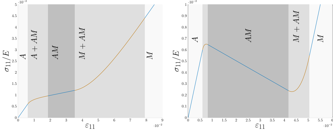
Figure 2: Stress-strain curve for a model texture with a density \tilde{\rho} = 1/(\eta^+ - \eta^-) ; \eta^+ = 0.05 , t = 0 , \gamma = 0.0003 , g_0 = 0.001 , b = 0.4 . Cases \eta^- = 0.02 (left) and \eta^- = 0.04 (right).
