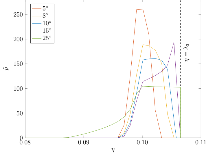
Figure 6: Densities \tilde{p} for \langle 111 \rangle \parallel \mathbf{u}_1 textures with different wobble. Case of NiTi.
