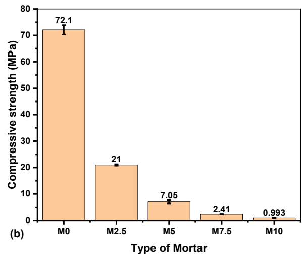
Fig. 13 – Mechanical properties of the different mortars at 28 days: (a) Flexural and (b) compressive strengths.
