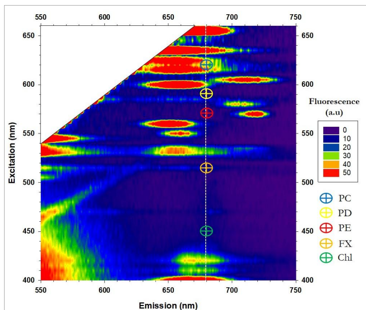
Figure 3 Lake Champs raw water fluorescence EEM and BBE Fluoroprobe sensor emission wavelength (680 nm) for pigment fluorescence detection; with Phycocyanin (PC), Peridinin (PD), Phycoerythrin (PE), Fucoxanthin (FX) and Chlorophylls (Chl).
