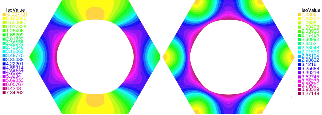
Figure 15: Maps of the energy density w_2/\sigma_2\|\bar{e}\|^{m+1} (left) and symmetrized energy density w_{2,sym}/\sigma_2\|\bar{e}\|^{m+1} (right) for the optimized inclusion in a periodic hexagonal cell with m = 2 , c_1 = 0.4 , \theta = 0 .
