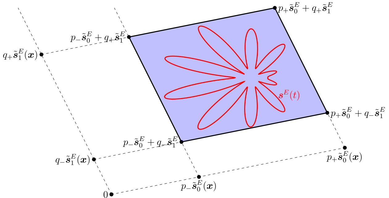
Figure 12: Pointwise bound on the radius \gamma(t) of the curve t \mapsto \mathbf{s}^E(\mathbf{x}, t) in the case of 2 loadings parameters.
