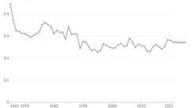
Figure 10: Vietnam annual fossil fuels&industry CO 2 emissions and its Kaya decomposition. CO_2 \text{ emissions} = \text{Population} * \text{PPP GDP} * \text{energy intensity} * \text{carbon intensity} . Source: Our World in Data, accessed 2023-01-10.
