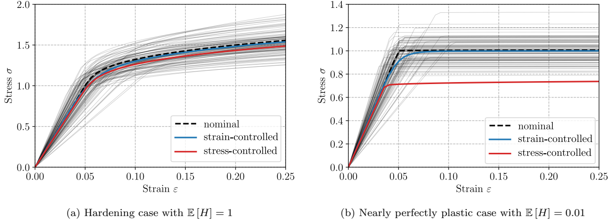
Figure 2: Effective behavior of a stochastic hardening elastoplastic material with strain-controlled (31) and stress-controlled (33) formulations. The black dashed line corresponds to the nominal deterministic case where all parameters take their average value. Thin black lines correspond to 100 independent realizations of the stochastic behavior.
