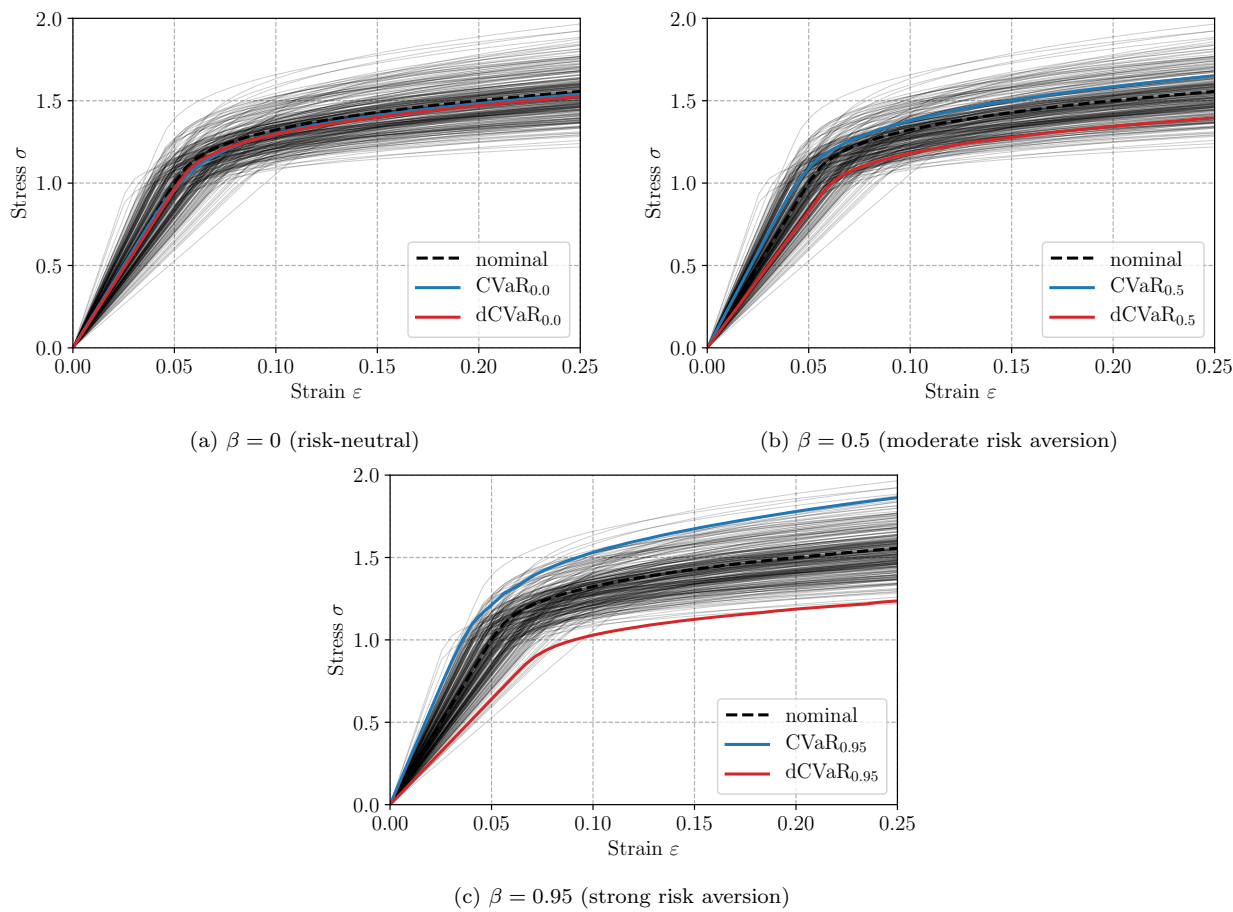
Figure 5: Optimistic (CVaR) and pessimistic (dCVaR) effective behaviors of a stochastic elastoplastic behavior (hardening case with \mathbb{E}[H] = 1 ) for various values of the risk aversion level \beta .
