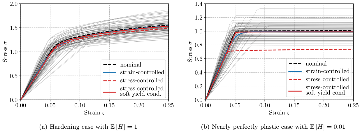
Figure 3: Effective behavior of a stochastic hardening elastoplastic material using the strain-controlled (31) and stress-controlled (33) formulations as well as the stress-controlled formulation (36) with a soft yield condition.
