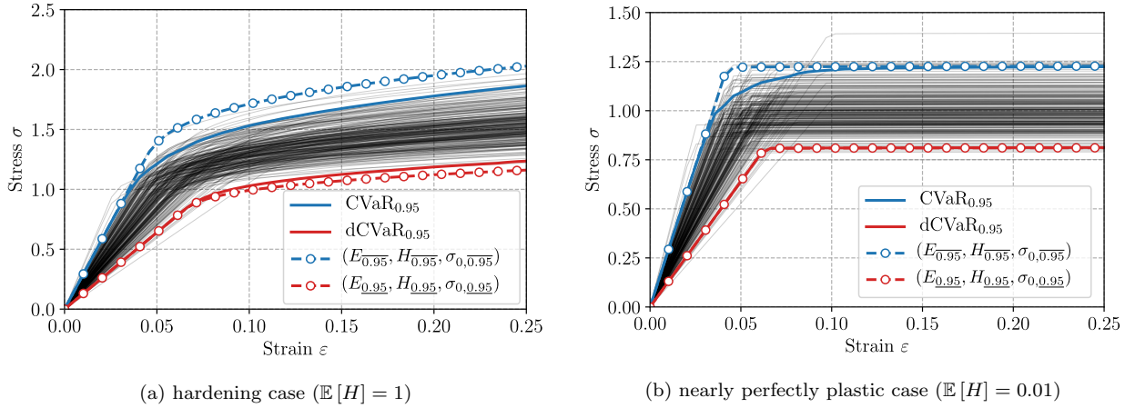
Figure 7: Comparison with elastoplastic behaviors associated with optimistic/pessimistic values of the material parameters ( \beta = 0.95 ).
