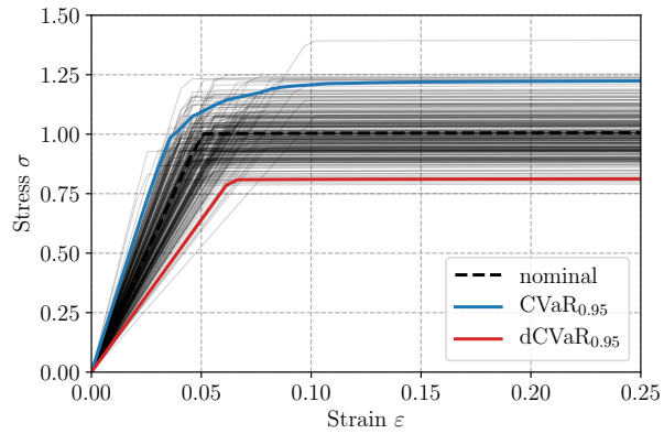
(c) \beta = 0.95 (strong risk aversion)
