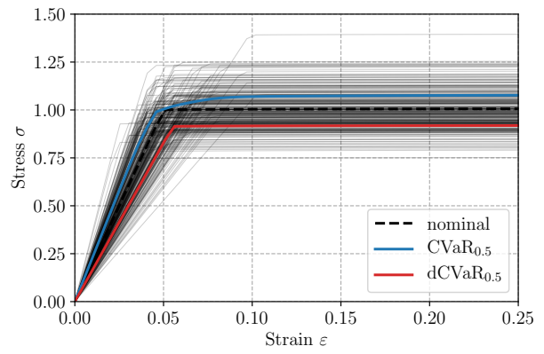
(b) \beta = 0.5 (moderate risk aversion)
