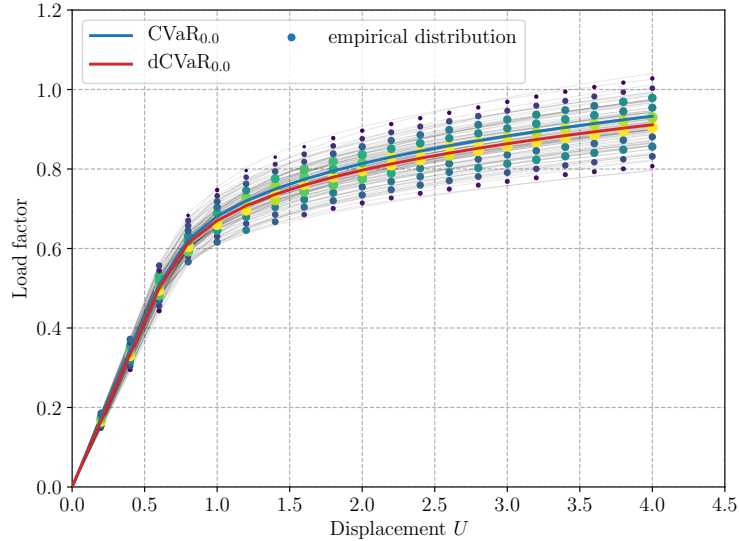
Figure 10: Risk-neutral \beta = 0 structural responses using the primal CVaR measure (91) and the dual dCVaR measure (94). Colored symbols indicate the empirical distribution of the structural response for fixed values of the imposed displacement. Color and size of the marker denote the frequency of the observed response.
