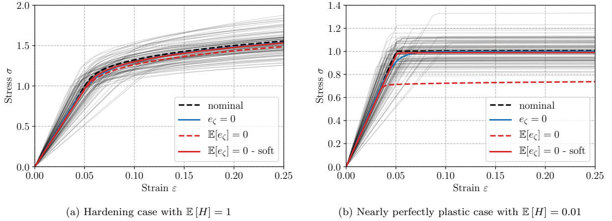
Figure 3: Effective behavior of a stochastic hardening elastoplastic material using the soft constraint formulations (39).
