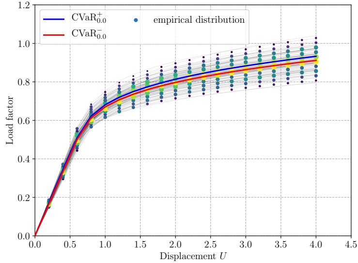
Figure 10: Risk-neutral \beta = 0 structural responses using the primal CVaR measure (99) and the dual dCVaR measure (102). Colored symbols indicate the empirical distribution of the structural response for fixed values of the imposed displacement. Color and size of the marker denote the frequency of the observed response.
