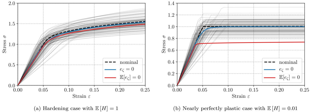
Figure 2: Effective behavior of a stochastic hardening elastoplastic material. The black dashed line corresponds to the nominal deterministic case where all parameters take their average value. Thin black lines correspond to 100 independent realizations of the stochastic behavior.
