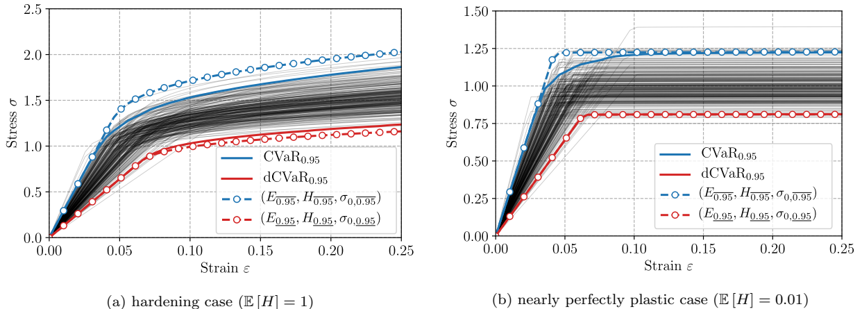
Figure 7: Comparison with elastoplastic behaviors associated with optimistic/pessimistic values of the material parameters ( \beta = 0.95 ).
