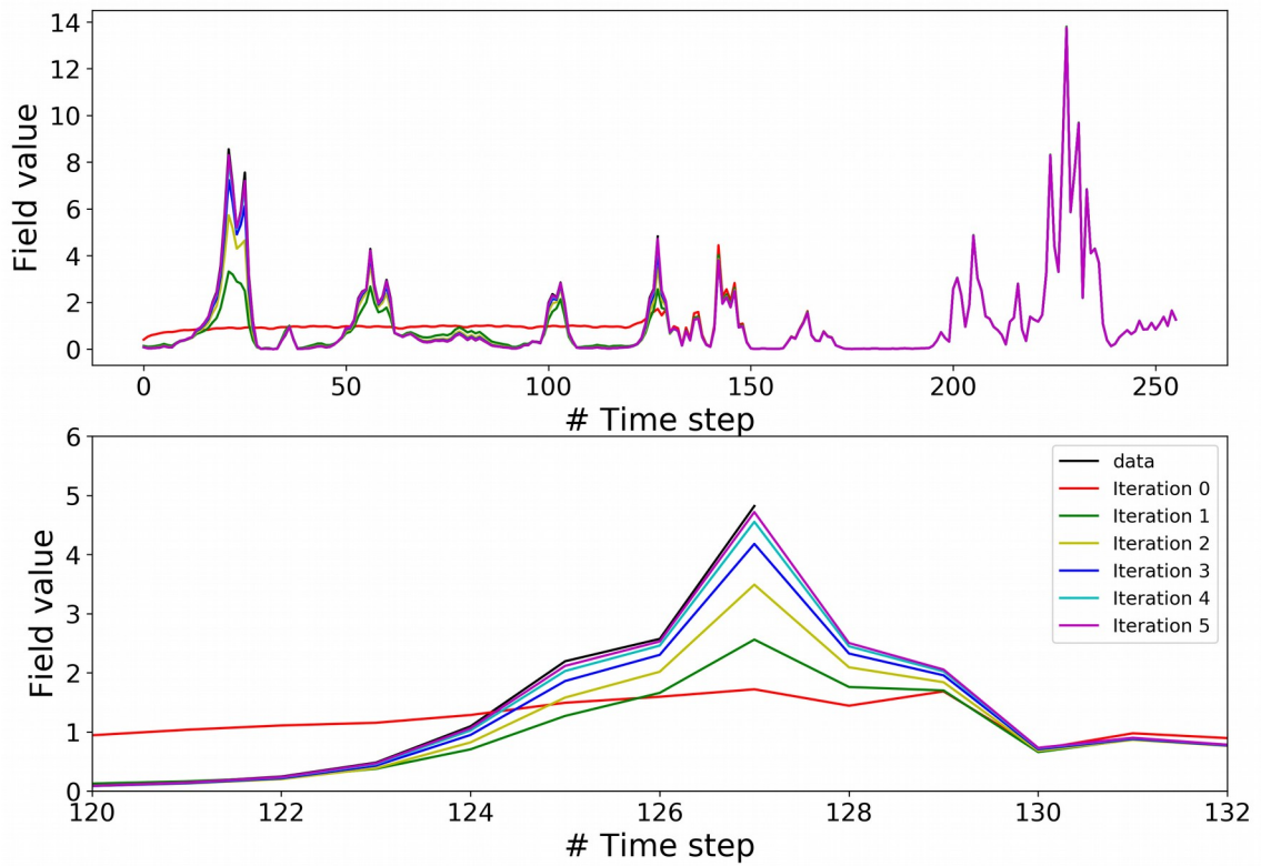
Figure 10: Illustration of the successive iterations of the process enabling to simulate a realistic follow-up of the initial series (of length 128) which is displayed in black. The lower part is simply a zoom of the upper one during the transition between the initial data and the stochastically generated second half.
