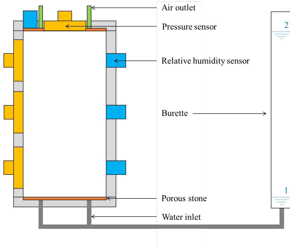
105 106 Figure 2. Sketch of the imbibition column, with the water levels associated to each phase of the experiment.
