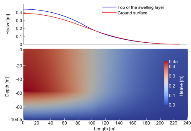
Fig. 2 Vertical displacement (heave) of the model domain after 1500 days simulation time
