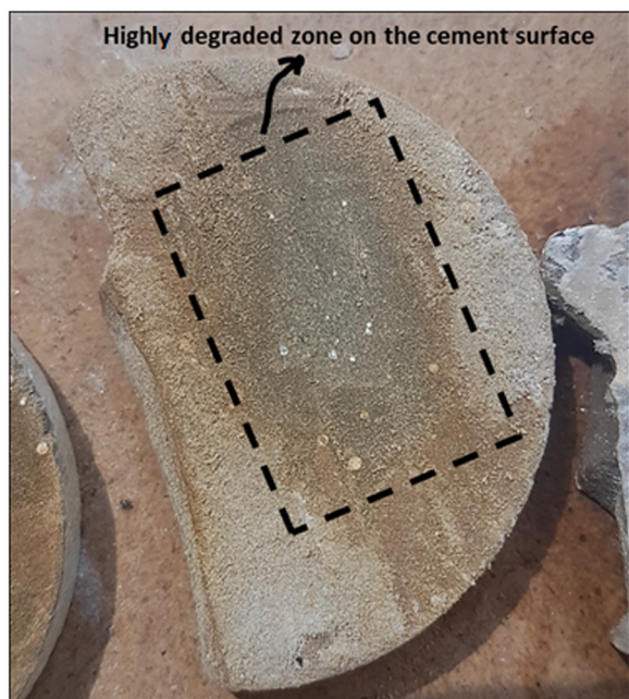
Fig. 4. Cement specimen after carbonation for 30 days at 20 MPa and 90°C.
