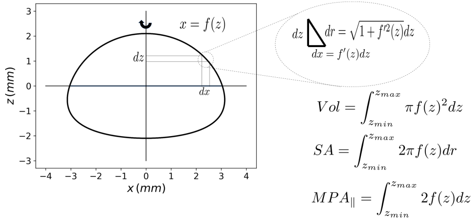
Figure 1. Illustration of how the volume (Vol), the surface area (SA) and the mean projected longitudinal cross-sectional area (MPA || ) of the particle used in this paper can be computed via integral calculus. The drop is actually a solid of revolution around the “z” axis.
