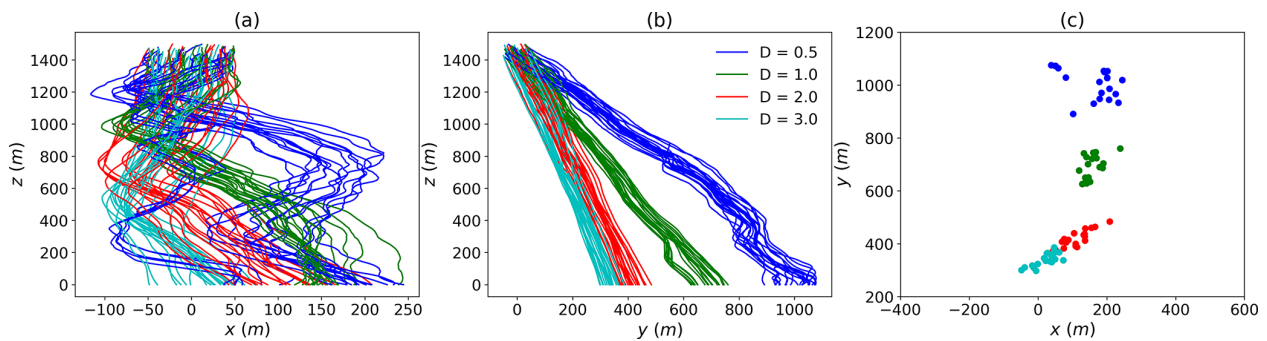
Figure 11. (a, b) Trajectories of drops of various sizes falling from a 100\text{ m}^3 cubic voxel centred on a (0, 0, 1450) position, projected on the (x, z) and (y, z) plane, respectively. The low wind event is used. For each size, the 20 drops are dropped every 15 s (hence over a total duration of 5 min). A single realization of the wind shift field is used. (c) Position of the ground impact of the various drops.
