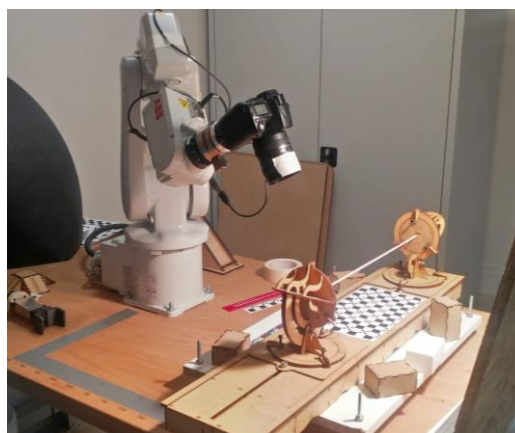
Figure 4: Robotized photogrammetry setup
