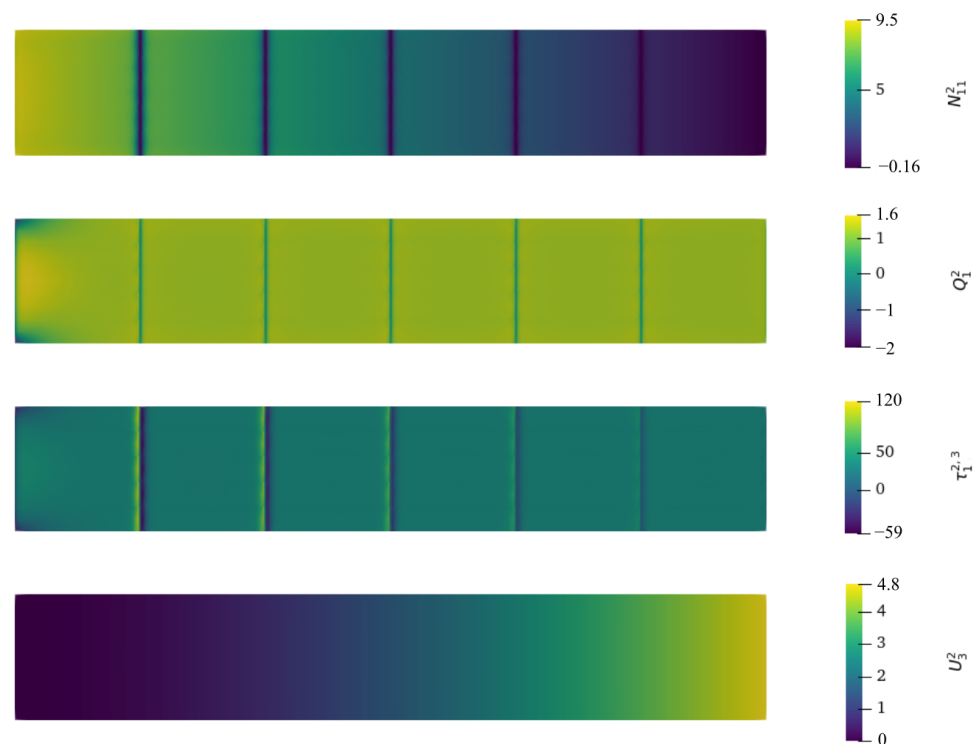
Figure 13. Generalized stresses and vertical displacement fields in layer 2 ( N_{11}^2 , Q_1^2 in MPa/m, \tau_{12}^{2,3} in MPa, U_3^2 in m).
