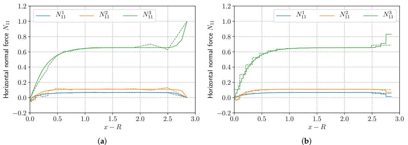
Figure 11. Evolution of N_{11} [MPa/m] along the plate length for a coarse (dotted line) and a fine (solid line) mesh. (a) N_{11} with the mixed ( p = 2 ) approach; (b) N_{11} with the displacement approach.
