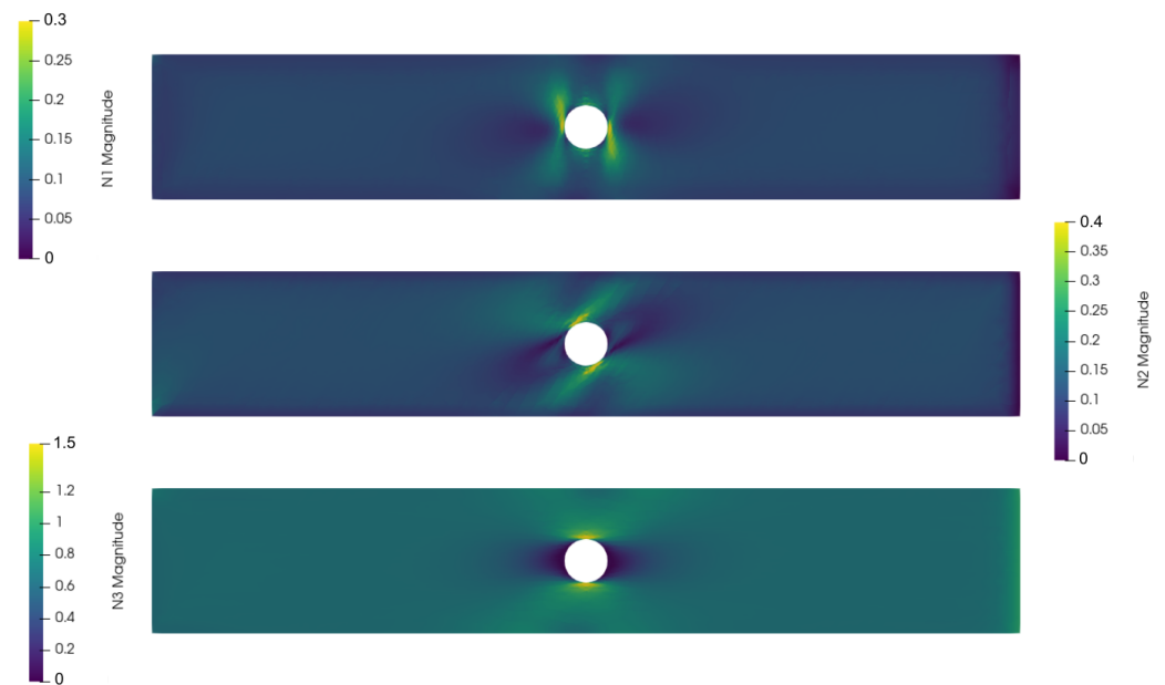
Figure 10. Magnitude \sqrt{N_{\alpha\beta}N_{\alpha\beta}} [MPa/m] in layers 1, 2, and 3.
