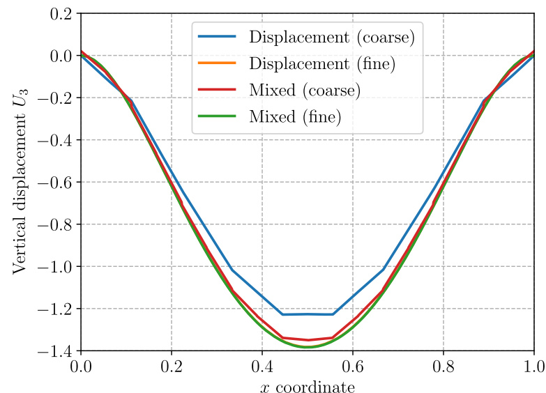
Figure 7. Vertical deflection U_3 [m] for the thin plate case (both solutions in the fine mesh case are superimposed).
