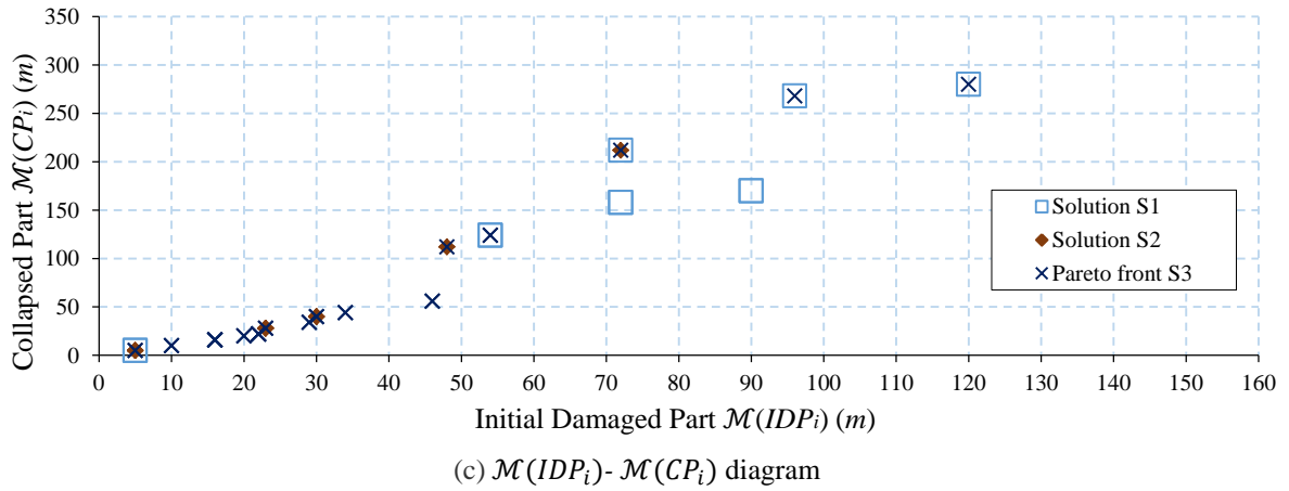
Figure 9. Pareto fronts S1, S2 and S3 in (a) E_i - DFP_i diagram, (b) M(IDP_i) - DFP_i diagram, and (c) M(IDP_i) - M(CP_i) diagram.
