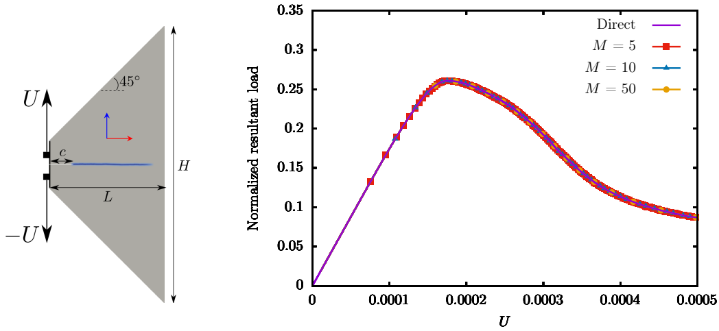
Figure A.24: (a) Geometry of the trapezium structure loaded in mode I and resulting stable crack path. The dimensions of the trapezium are L = 5 mm, H = 12 mm and the notch length is c = 1 mm. (b) Evolution of normalized resultant load vs displacement imposed to the trapezium ends obtained with direct and hybrid resolution strategies. The regularization length scale is equal to \ell = 0.02 mm and the cleavage energy is G_c = 10^{-3} J/m 2 for both damage mechanisms. Isotropic elasticity is considered with E = 200 GPa and \nu = 0.3 .
