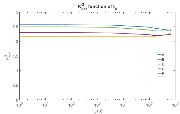
Figure 8: k_{def}^G estimate as function of t_0 .
