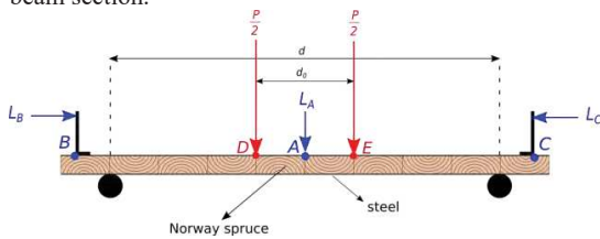
Figure 1: Four-point bending configuration on a sandwich beam
