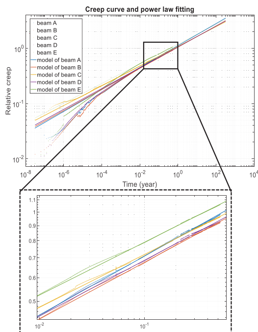
Figure 7: Rolling-shear relative creep curves and power law fittings.
