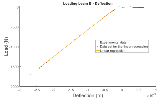
Figure 6: Applied force as a function of the mid-span deflection f_A
