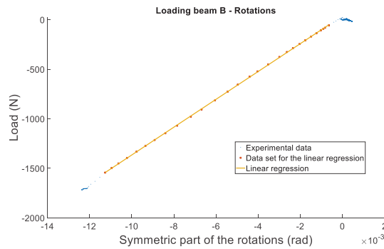
Figure 5: Applied force as a function of the rotation at support \Delta\varphi
