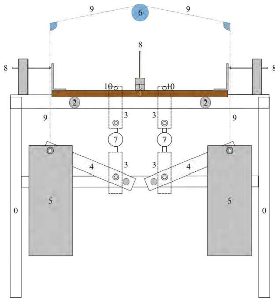
Figure 3: Framework
