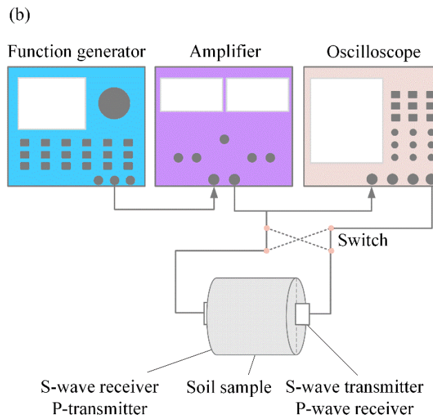
Fig. 3. Set-up of bender element test: (a) photo of the set-up; (b) sketch of the set-up (after Wang et al., 2017).
