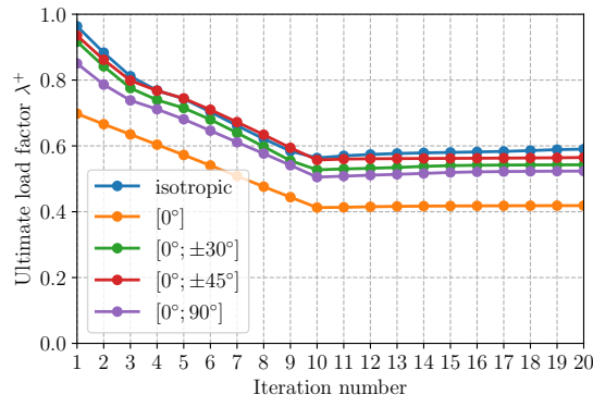
Figure 9: Evolution of the load-bearing capacity during the penalization procedure for the MBB example with discrete tensile orientations
