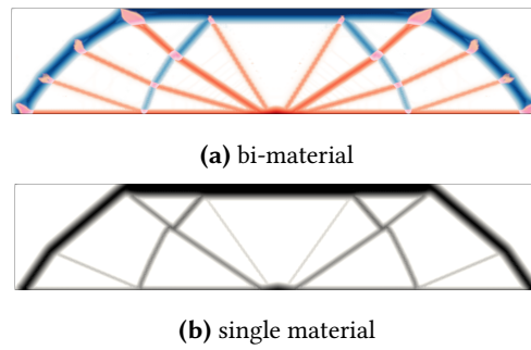
Figure 12: Asymmetric strengths f_c = 1, f_t = 10
