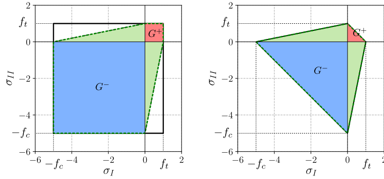
Figure 3: Splitting of a nominal strength criterion G (in black) into a purely compressive part G^- (in blue) and a purely tensile part G^+ (in red) and the corresponding convex hull \mathbf{conv}\{G^+, G^-\} (in green). Left: a Rankine strength criterion, right: a L_1 -Rankine strength criterion in the plane of principal stresses
