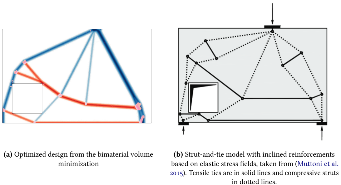
Figure 17: Comparison of the proposed methodology with strut-and-tie models with inclined reinforcements
