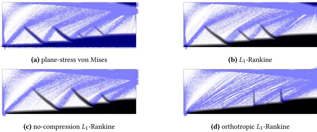
Figure 5: Reinforcement optimization of the MBB example for various reinforcement strength criteria: in black, reinforcement optimized density; in blue, principal compressive stress in the matrix phase.
