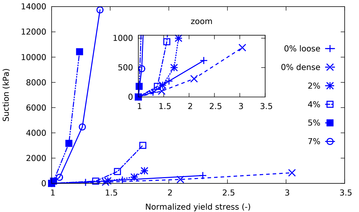
(b) Yield stress normalised with respect to saturated state
