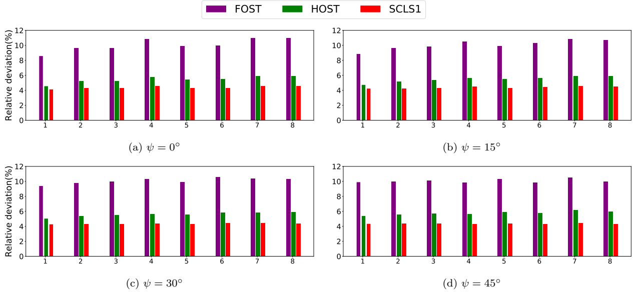
Figure 10: Relative error with respect to the three-dimensional model of the frequency parameter \lambda = \omega a^2 \sqrt{\rho/E_2 h^2} for a skew laminate plate (45/ - 45/45/ - 45); a/h = 10 , E_1/E_2 = 40 , G_{12} = 0.6E_2 , G_{13} = G_{23} = 0.5E_2 , \nu_{12} = \nu_{13} = \nu_{23} = 0.25
