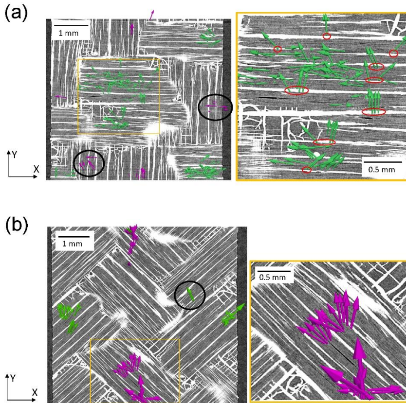
Figure 13. Principal vectors of the high-magnitude strains ( \epsilon_{max} > \epsilon^{thr} ) created at the last loading increment of (a) the 0/90 specimen and (b) the \pm 45 specimen. The vectors are shown in 3D, while the woven structure is shown through a 2D slice of the XCT image located at the strains under investigation. The vectors in the bundles of different orientations are distinguished by two different colours. The starting point of arrow is the position at which the strain is measured.
