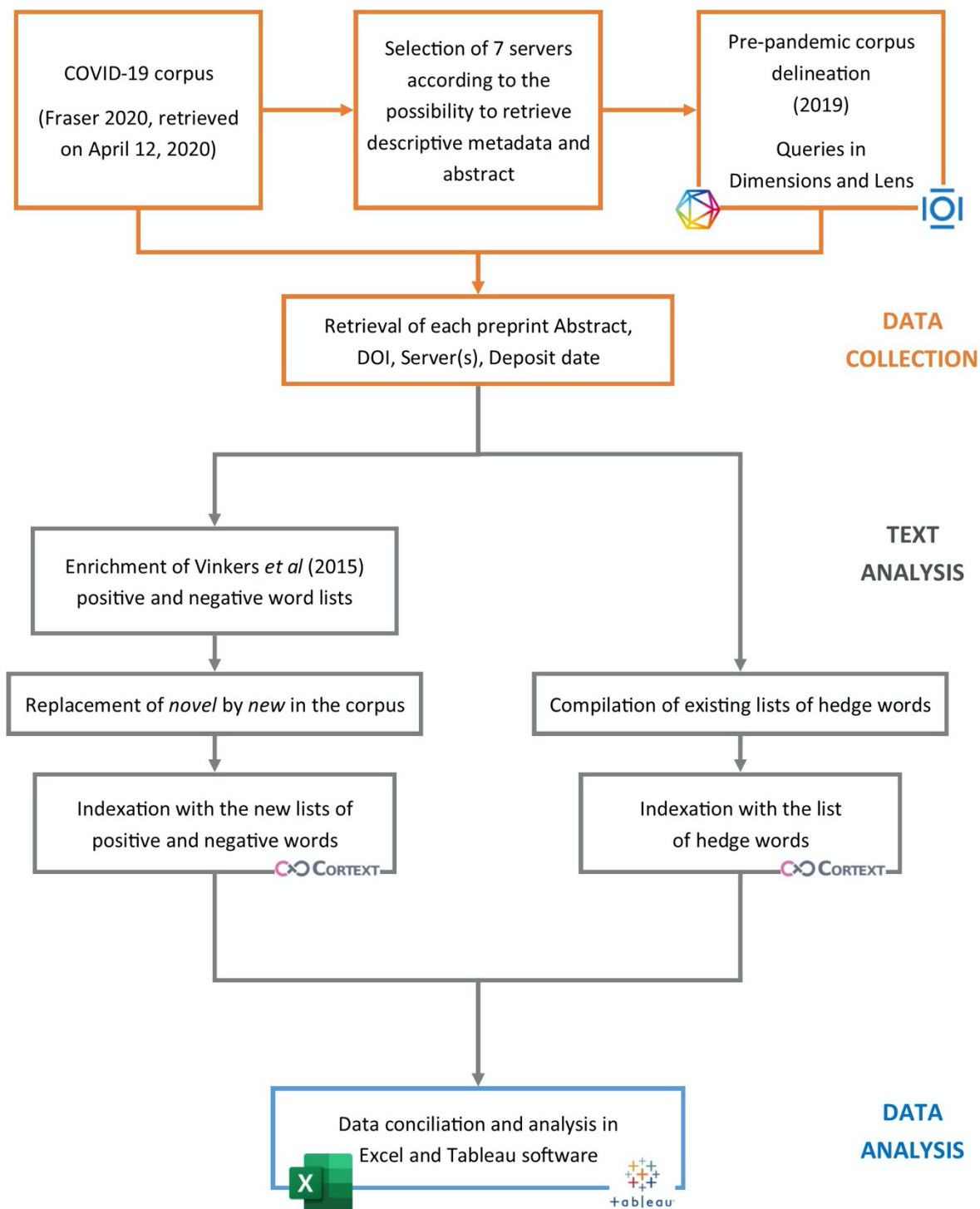
Fig 1. Study workflow
