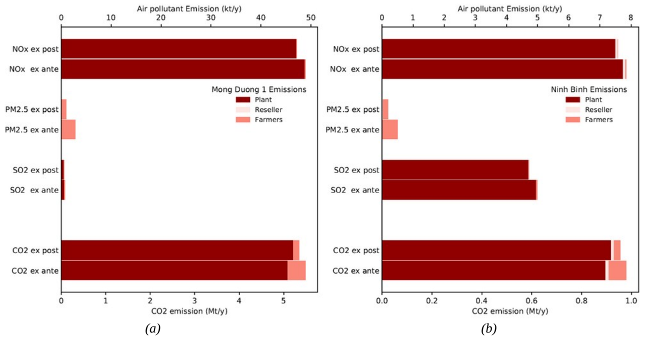
Figure 4: Pollutant emissions per year. (a) new plant case (Mong Duong 1-like), (b) old plant case (Ninh Binh-like). NO x , PM 2.5 , SO 2 on the top scale in kt/y, CO 2 on the bottom scale in Mt/y. Total emissions ex-post (with co-firing) are lower for all pollutants. Within each bar, the contribution of the three segments is shown. For example, the bottom pairs of broken bars show that CO 2 emissions at the plant are higher ex-post, but this is more than compensated by reductions of emissions by the farmers.
