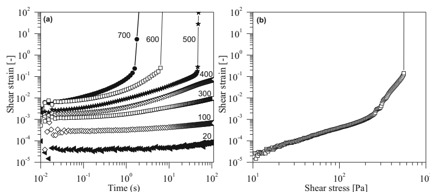
Fig. 12 Experiments performed with 10 wt% of wax in oil, T_i = 60^\circ\text{C} , 1^\circ\text{C/min} of cooling rate, T_f = 25^\circ\text{C} , and 10 min of resting time. a Shear strain as a function of time in the creep test. Before each plateau of stress, the sample is heated and cooled again using the same thermal history.
