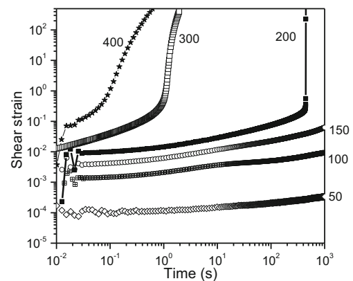
Fig. 3 Creep test performed after the same thermal history that was imposed in the experiments performed in Fig. 1 ( T_i = 60 °C, cooling rate 1 °C/min and T_f = 25 °C). For each test, the material is heated and cooled again in order to get the same initial state before each experiment. 8 wt% of paraffin in oil. Data from Andrade and Coussot (2019)
