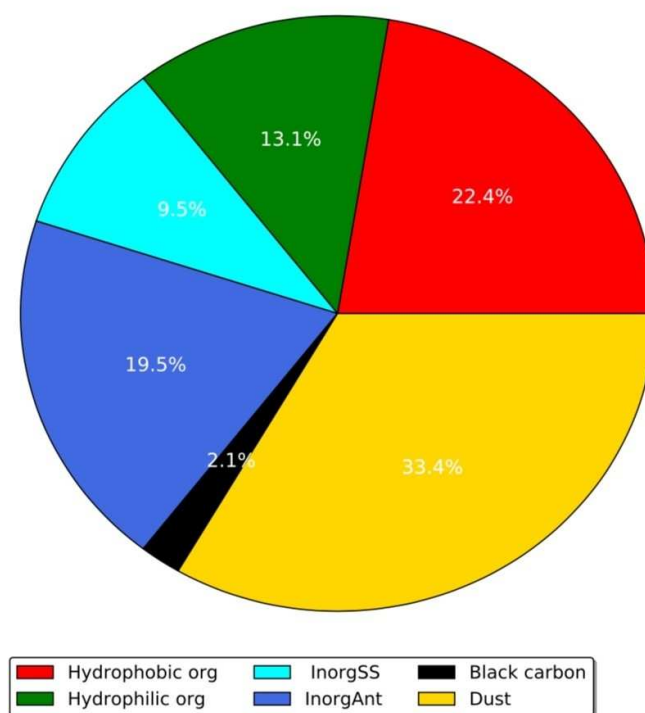
Figure 1: Mean composition of surface PM 10 concentration during the simulation over the Euro-Mediterranean region.
