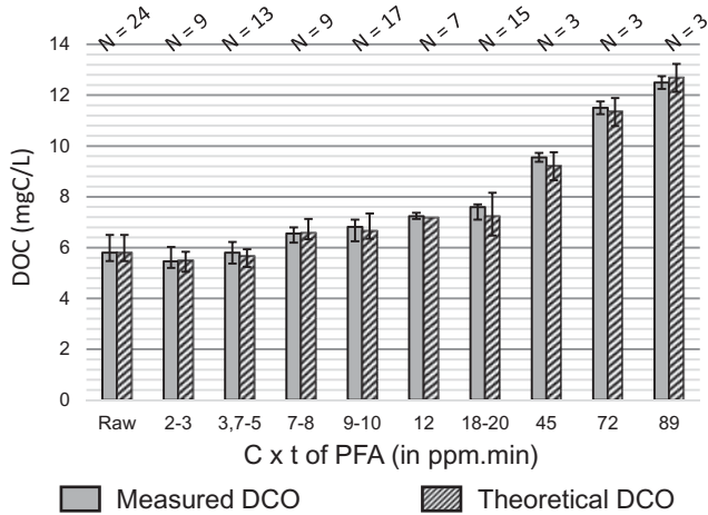
Figure 14 Impact of PFA injection at various C \times t on the dissolved organic carbon content of SEV WWTP discharge samples.
