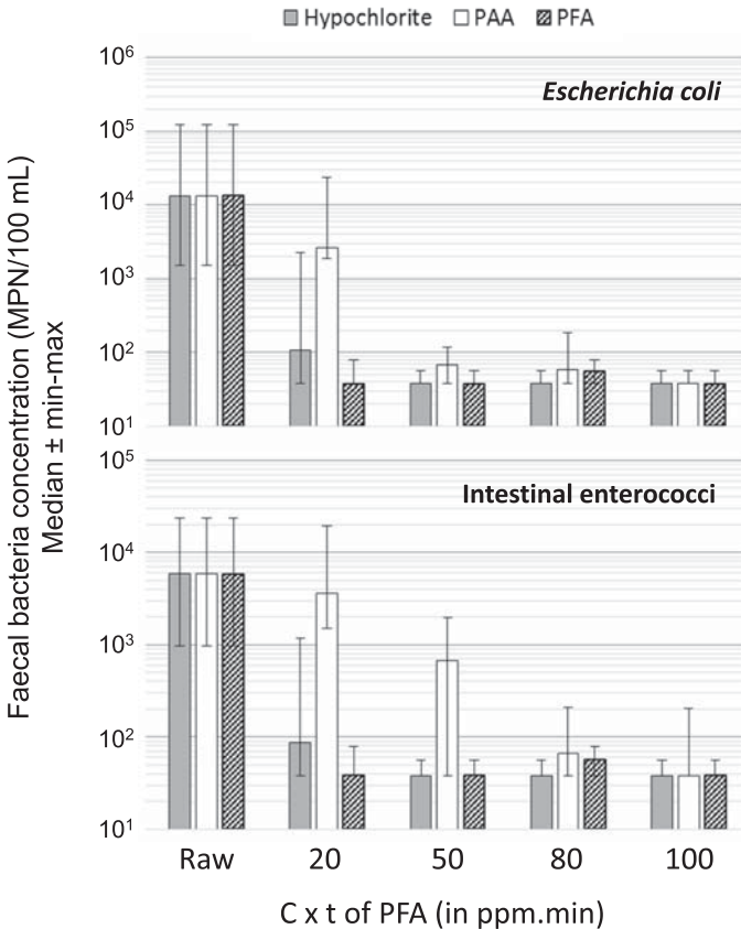
Figure 4 Batch scale comparison of faecal bacteria disinfection effectiveness of PFA, PAA and hypochlorite applied to SEV WWTP discharge (contact time: 10 min).
