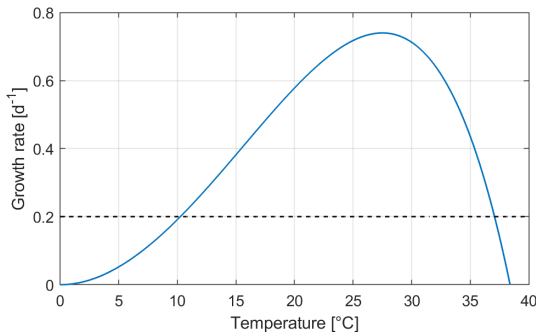
Figure 2. Thermal growth rate calculated after Eq. (7). The horizontal dashed line for GR = 0.2 \text{ d}^{-1} meets the curve at the temperature limits for the calculation of the GDDs (10 and 37^\circ\text{C} , respectively).
